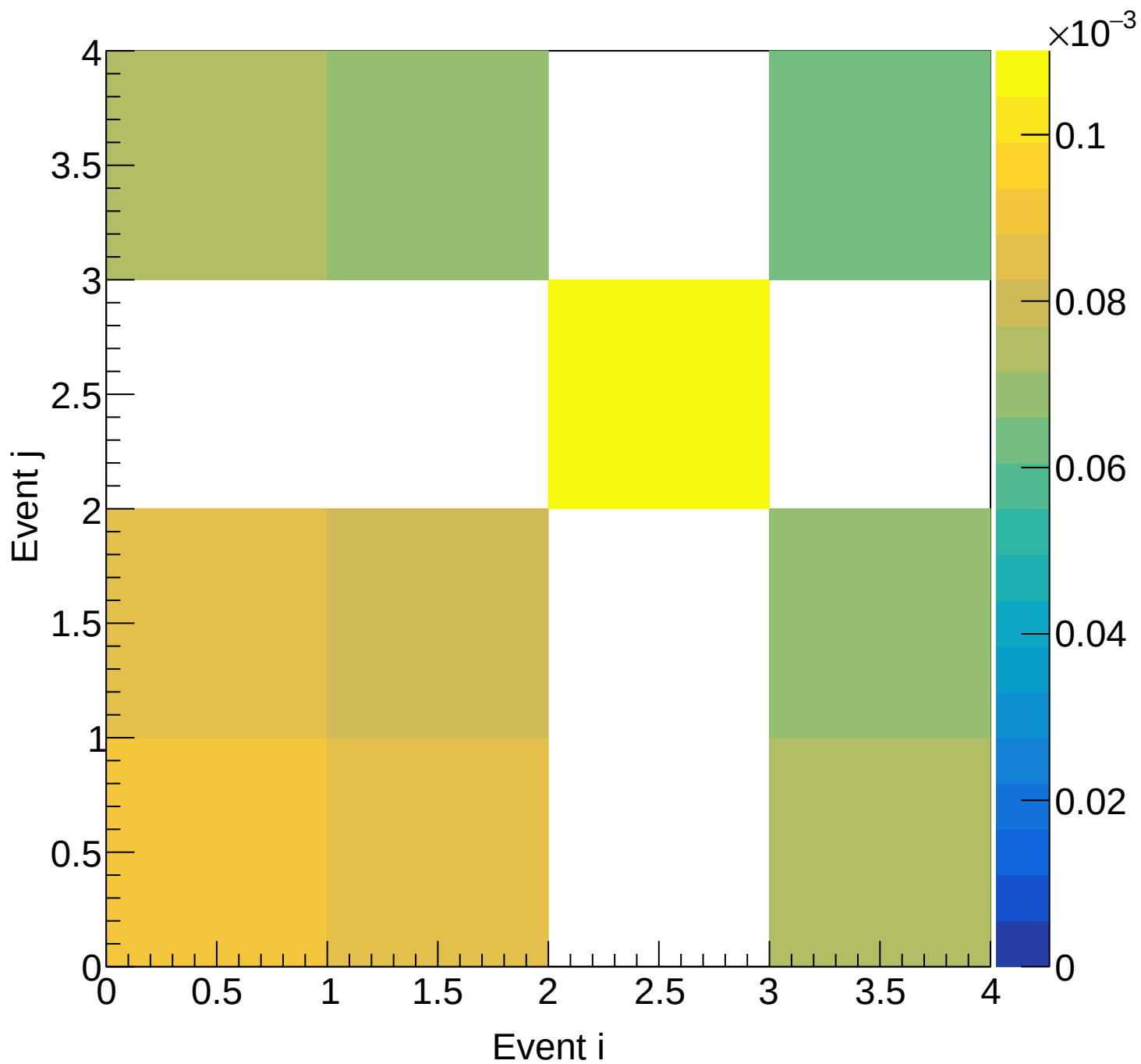
Flask (total) Covariance | M: [4.2, 4.5) xF: [0.65, 0.70)
