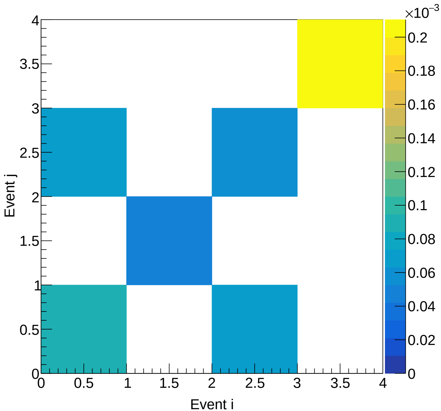
Flask (total) Covariance | M: [4.8, 5.1) xF: [0.65, 0.70)
