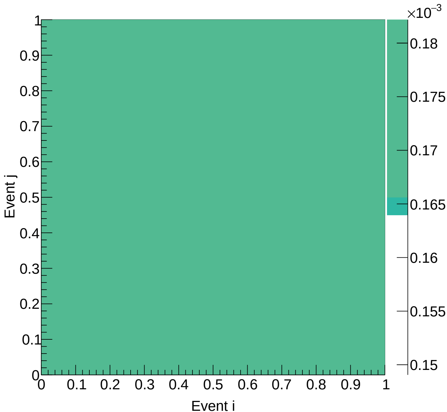
Flask (total) Covariance | M: [6.3, 6.6) xF: [0.65, 0.70)
