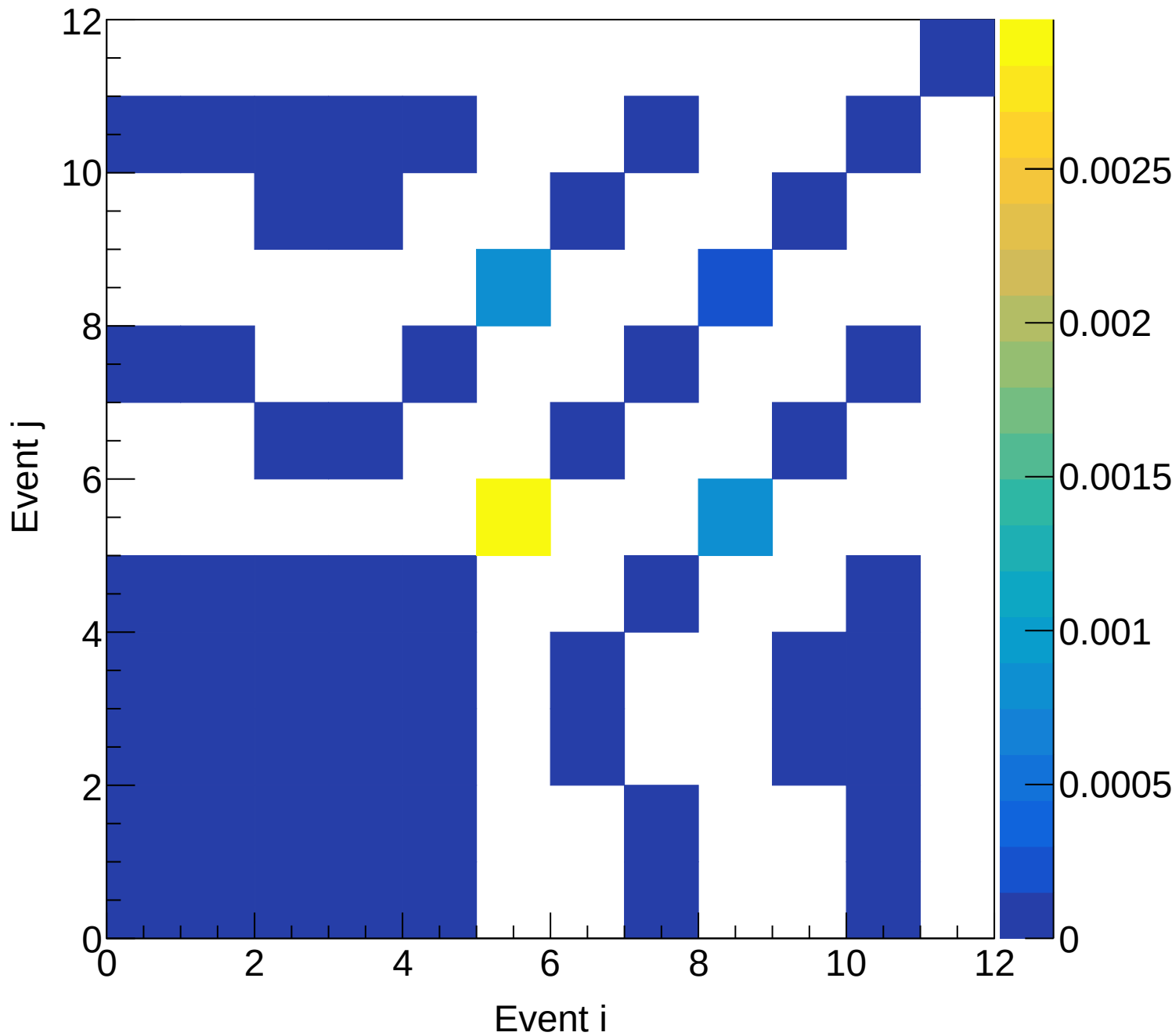
Flask (total) Covariance | M: [3.9, 4.2) xF: [0.70, 0.75)
