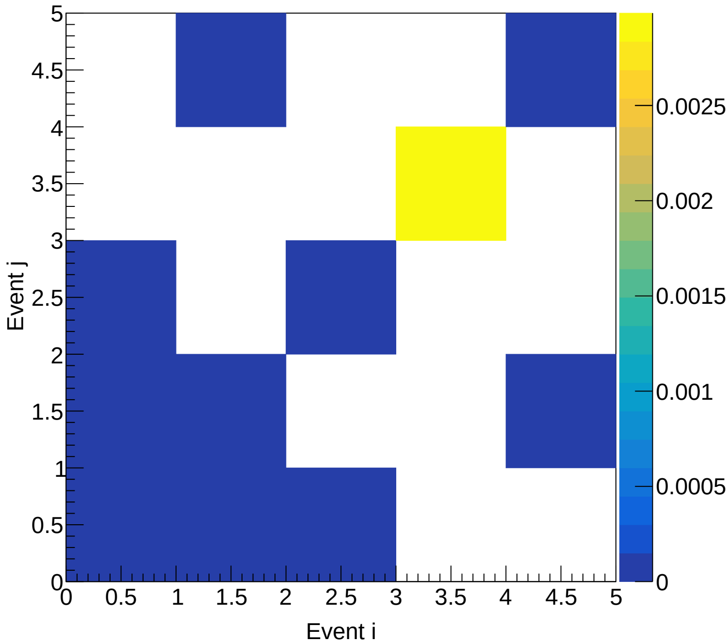
Flask (total) Covariance | M: [4.2, 4.5) xF: [0.70, 0.75)
