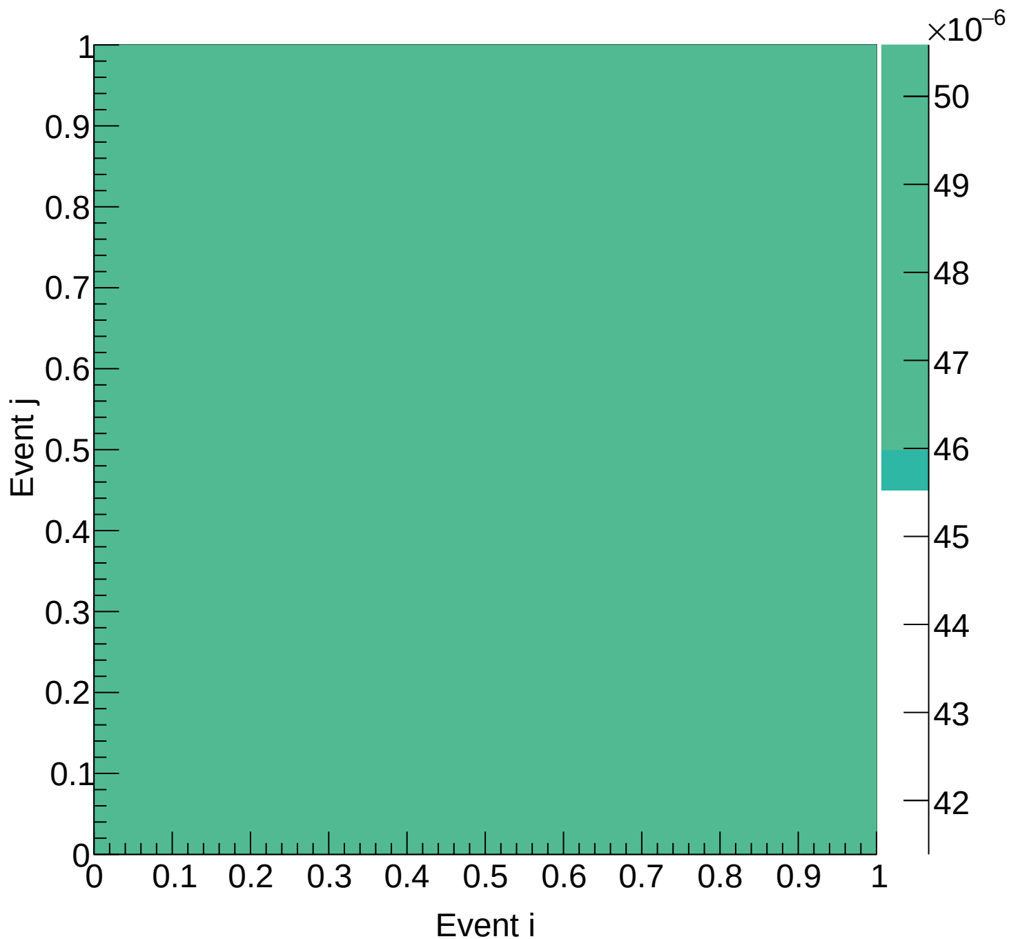
Flask (total) Covariance | M: [5.1, 5.4) xF: [0.70, 0.75)
