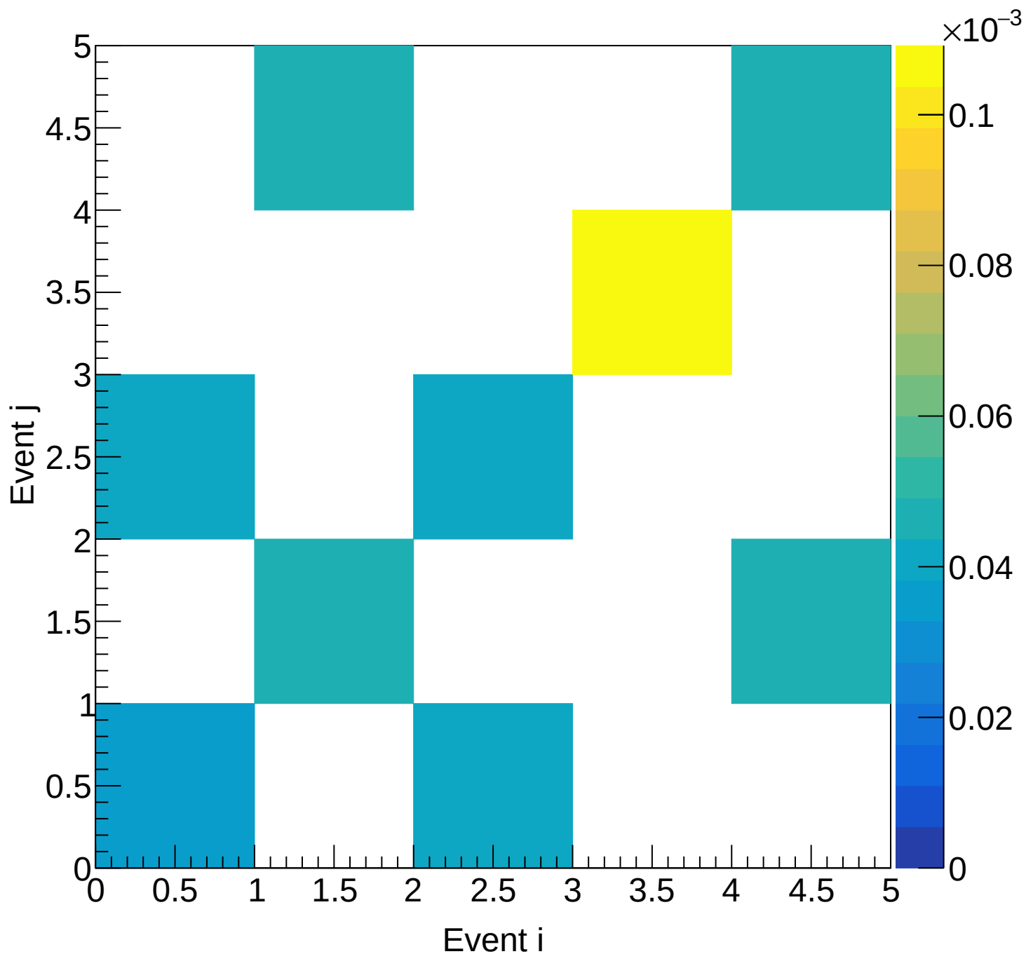
Flask (total) Covariance | M: [5.1, 5.4) xF: [0.00, 0.05)
