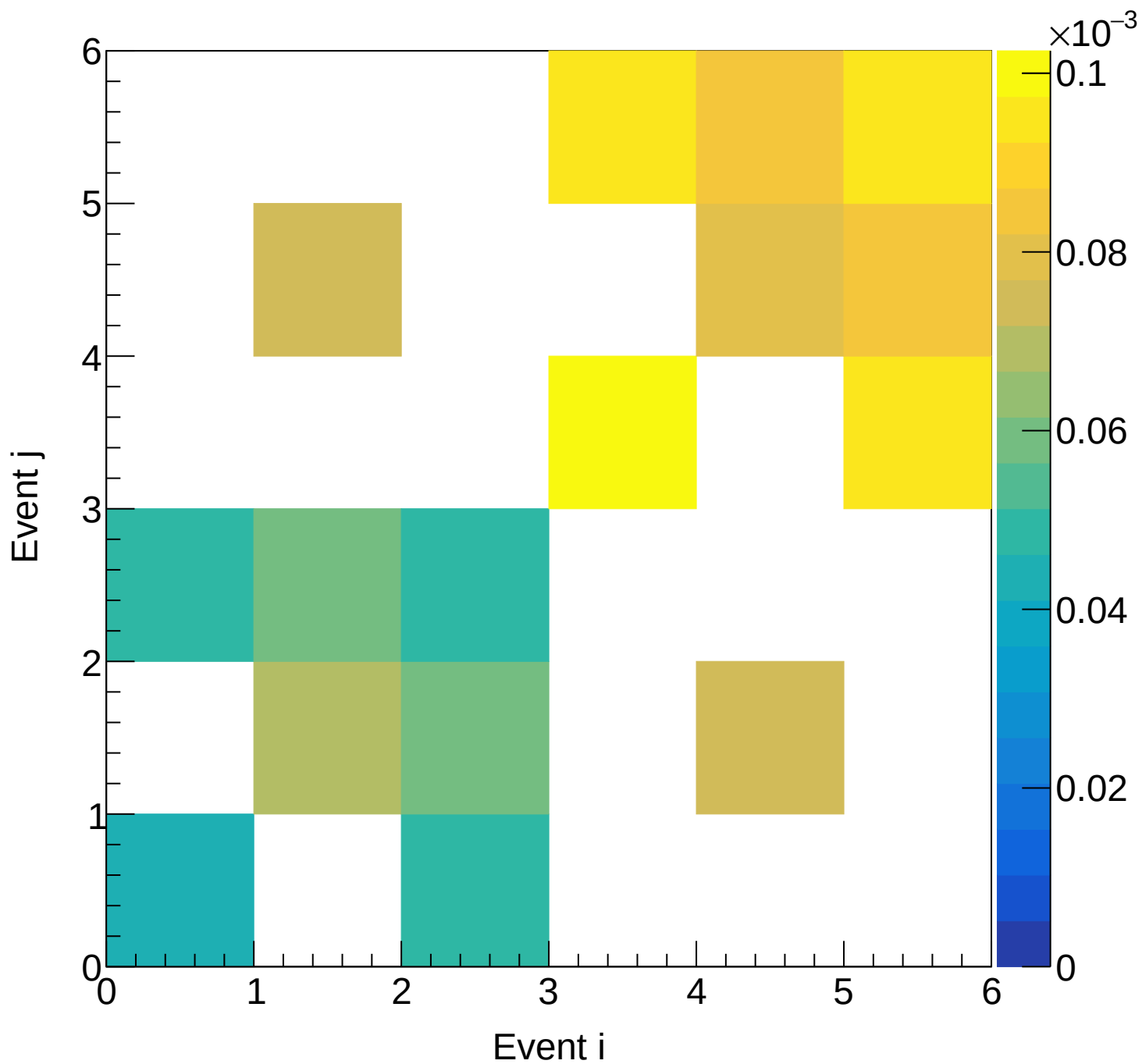
Flask (total) Covariance | M: [5.4, 5.7) xF: [0.00, 0.05)
