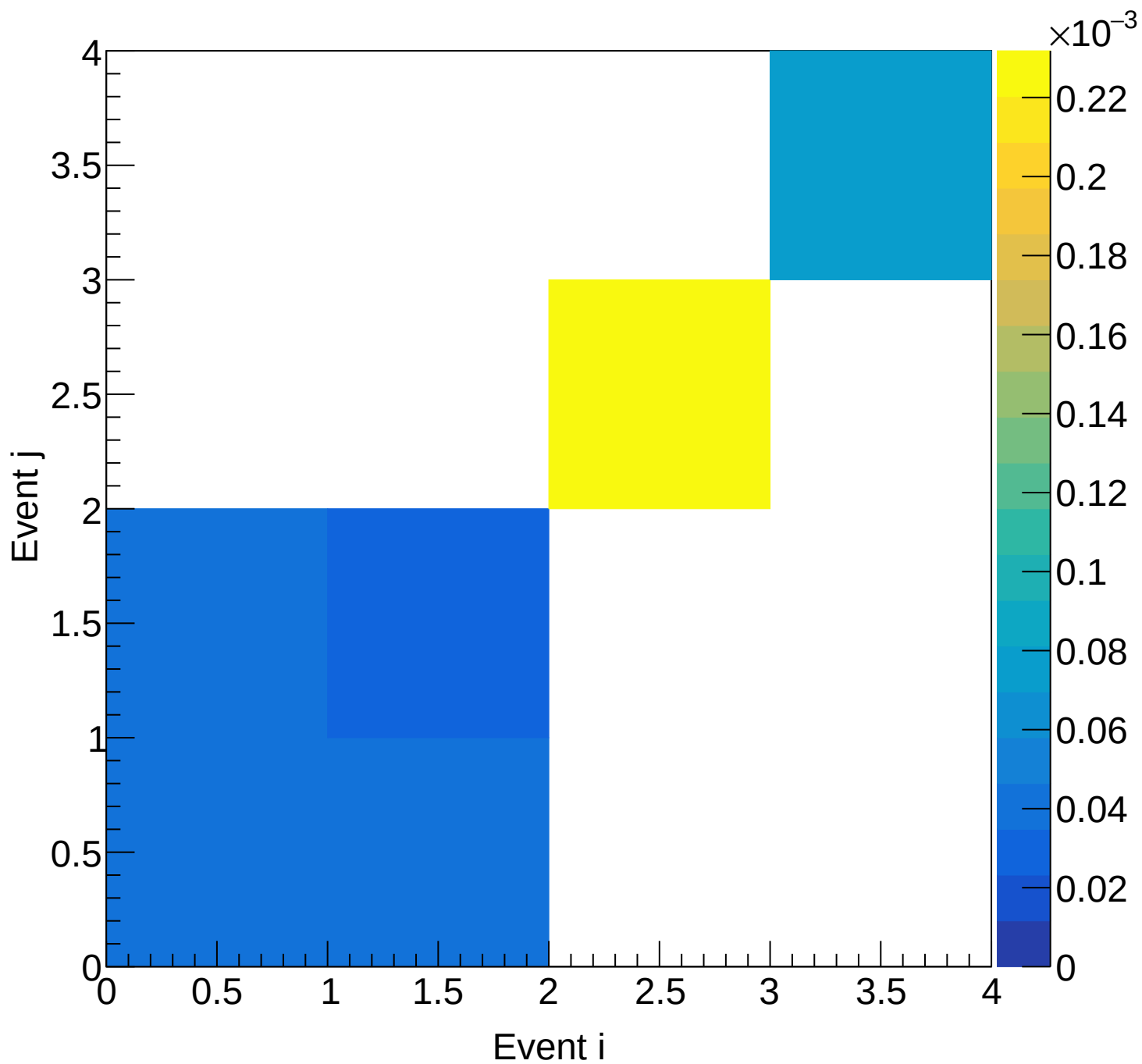
Flask (total) Covariance | M: [4.8, 5.1) xF: [0.05, 0.10)
