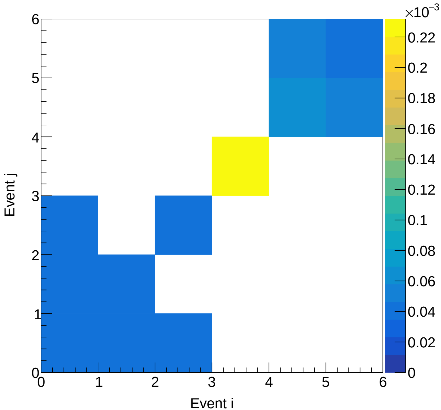
Flask (total) Covariance | M: [5.1, 5.4) xF: [0.05, 0.10)
