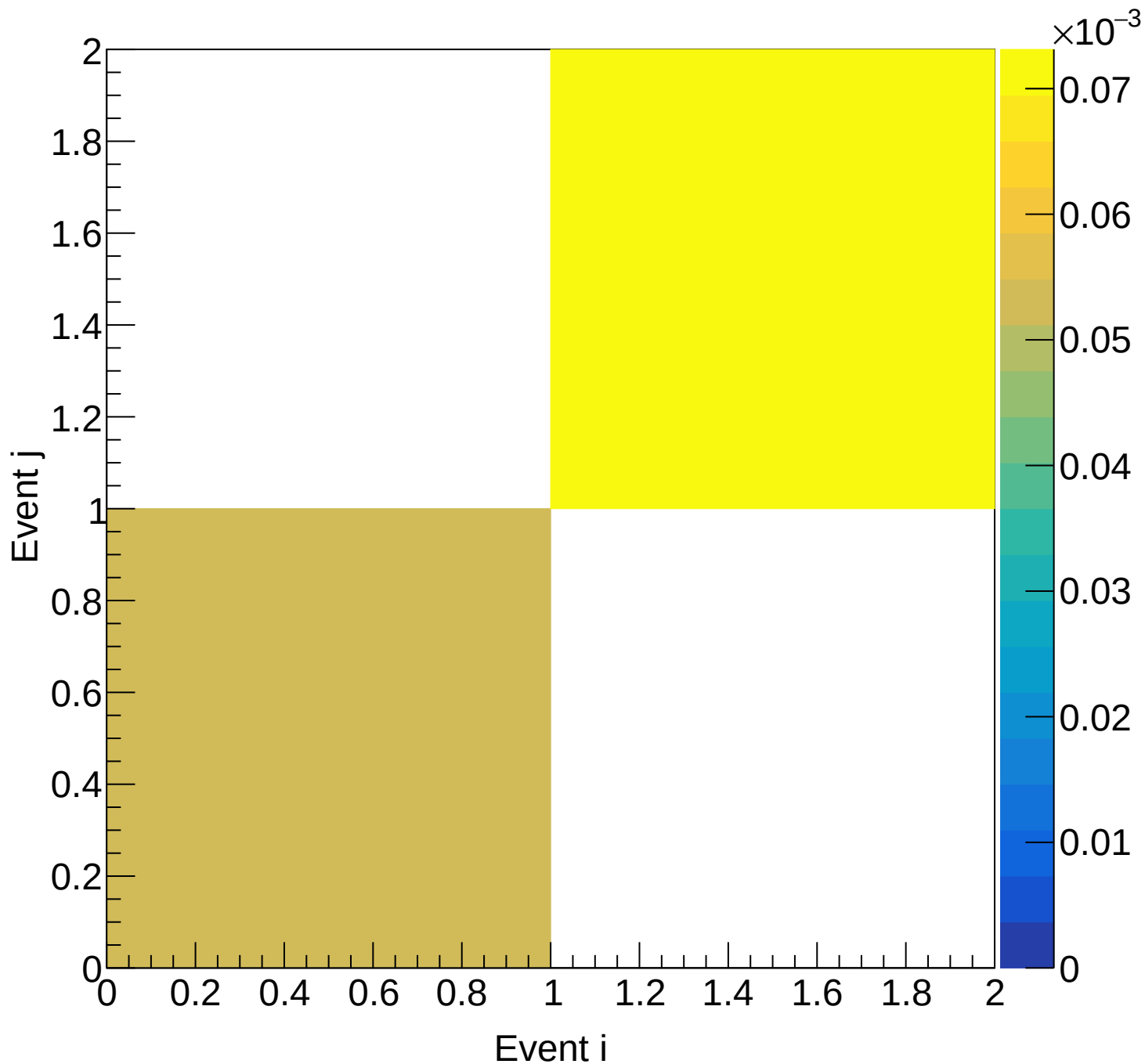
Flask (total) Covariance | M: [6.0, 6.3) xF: [0.05, 0.10)
