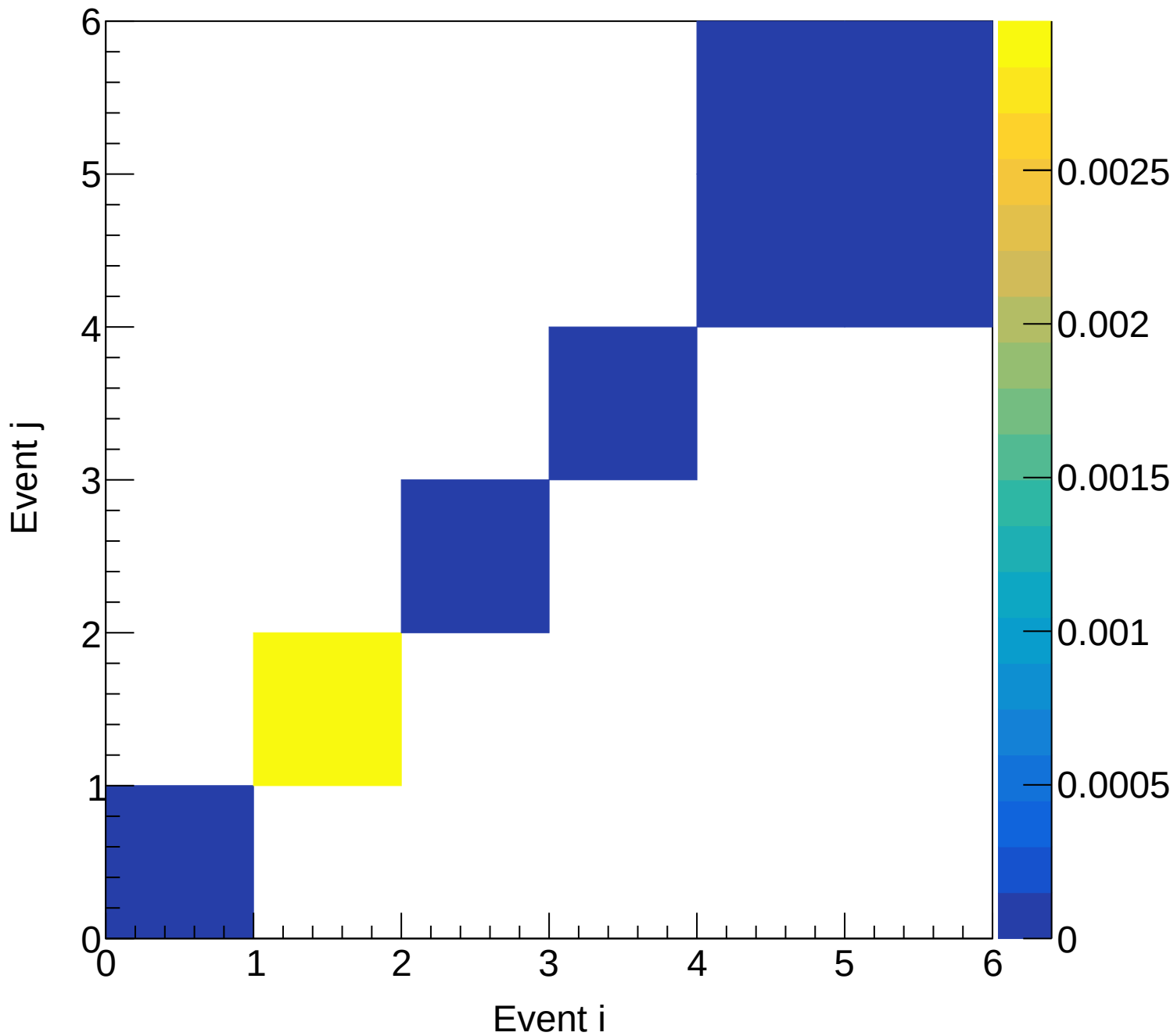
Flask (total) Covariance | M: [4.5, 4.8) xF: [0.10, 0.15)
