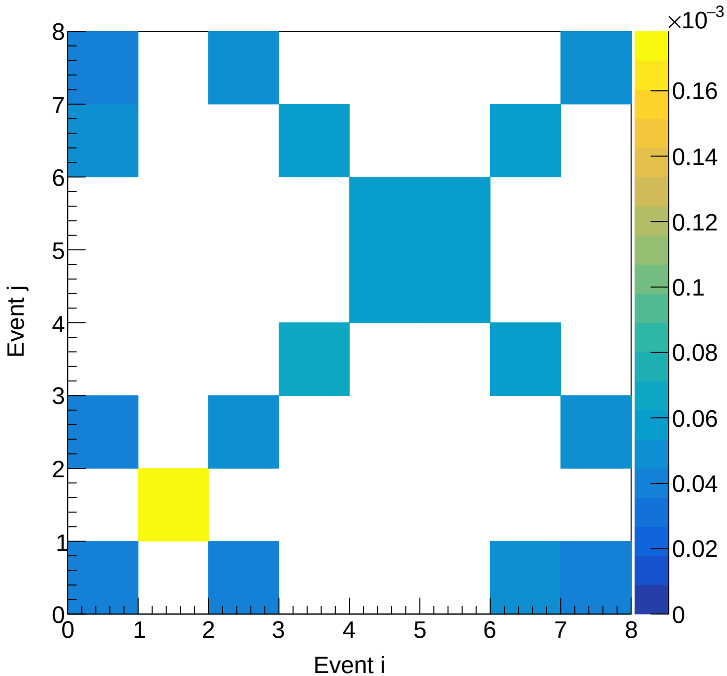
Flask (total) Covariance | M: [4.8, 5.1) xF: [0.10, 0.15)
