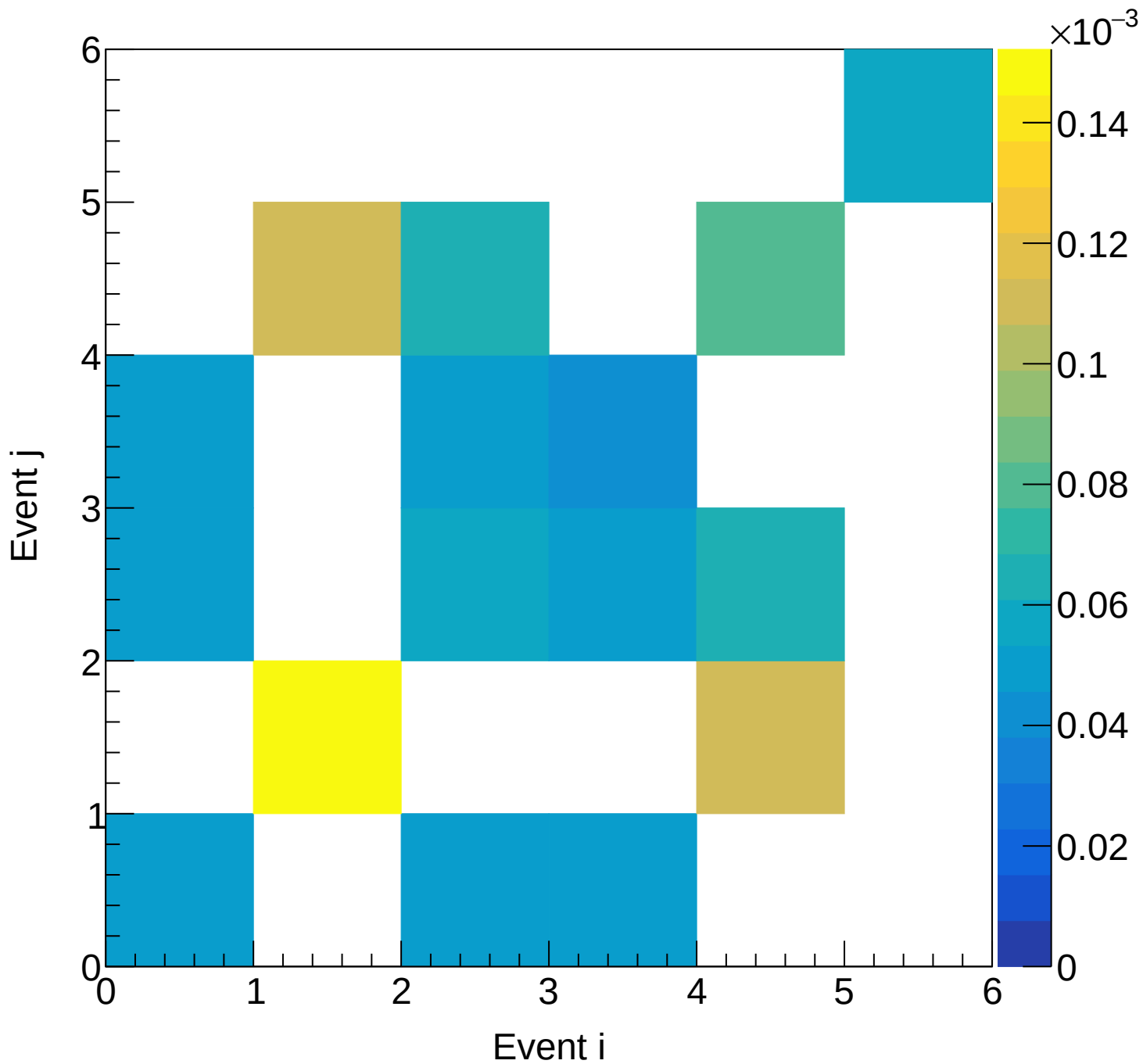
Flask (total) Covariance | M: [5.4, 5.7) xF: [0.10, 0.15)
