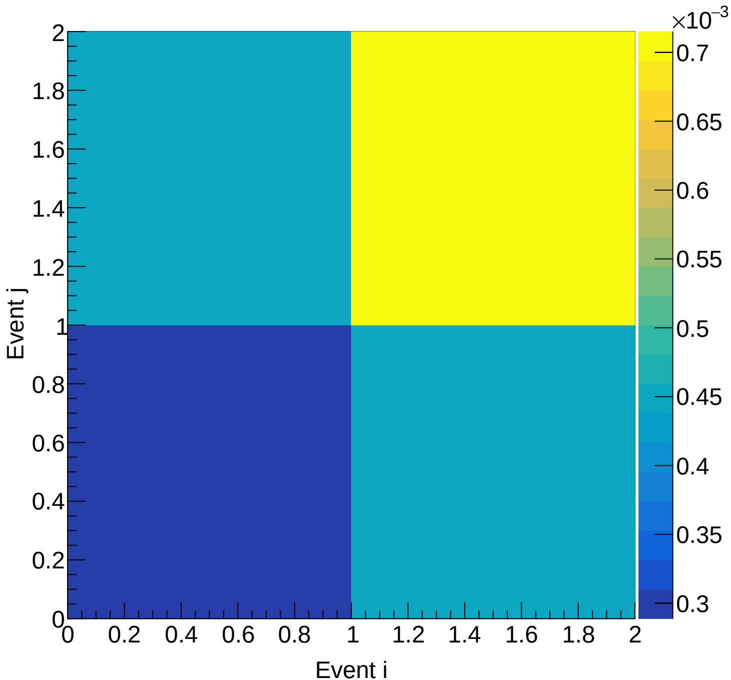
Flask (total) Covariance | M: [6.3, 6.6) xF: [0.15, 0.20)
