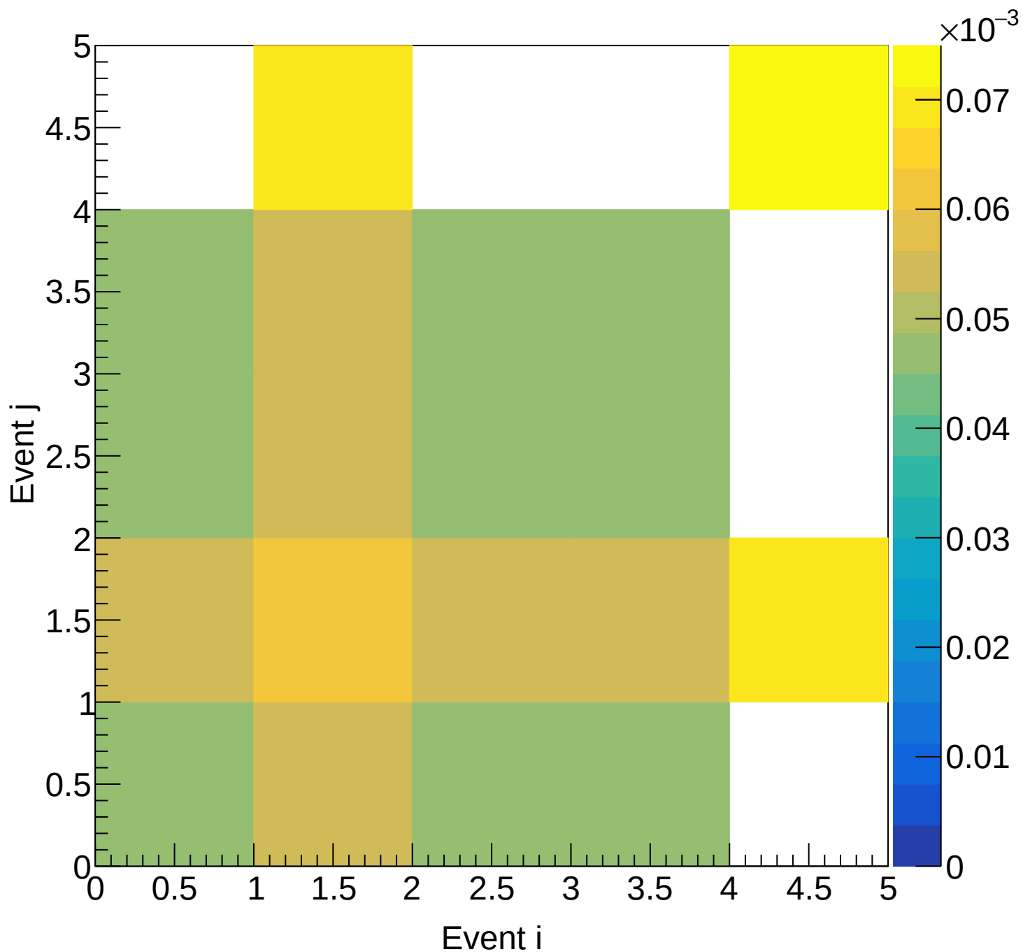
Flask (total) Covariance | M: [3.9, 4.2) xF: [0.15, 0.20)
