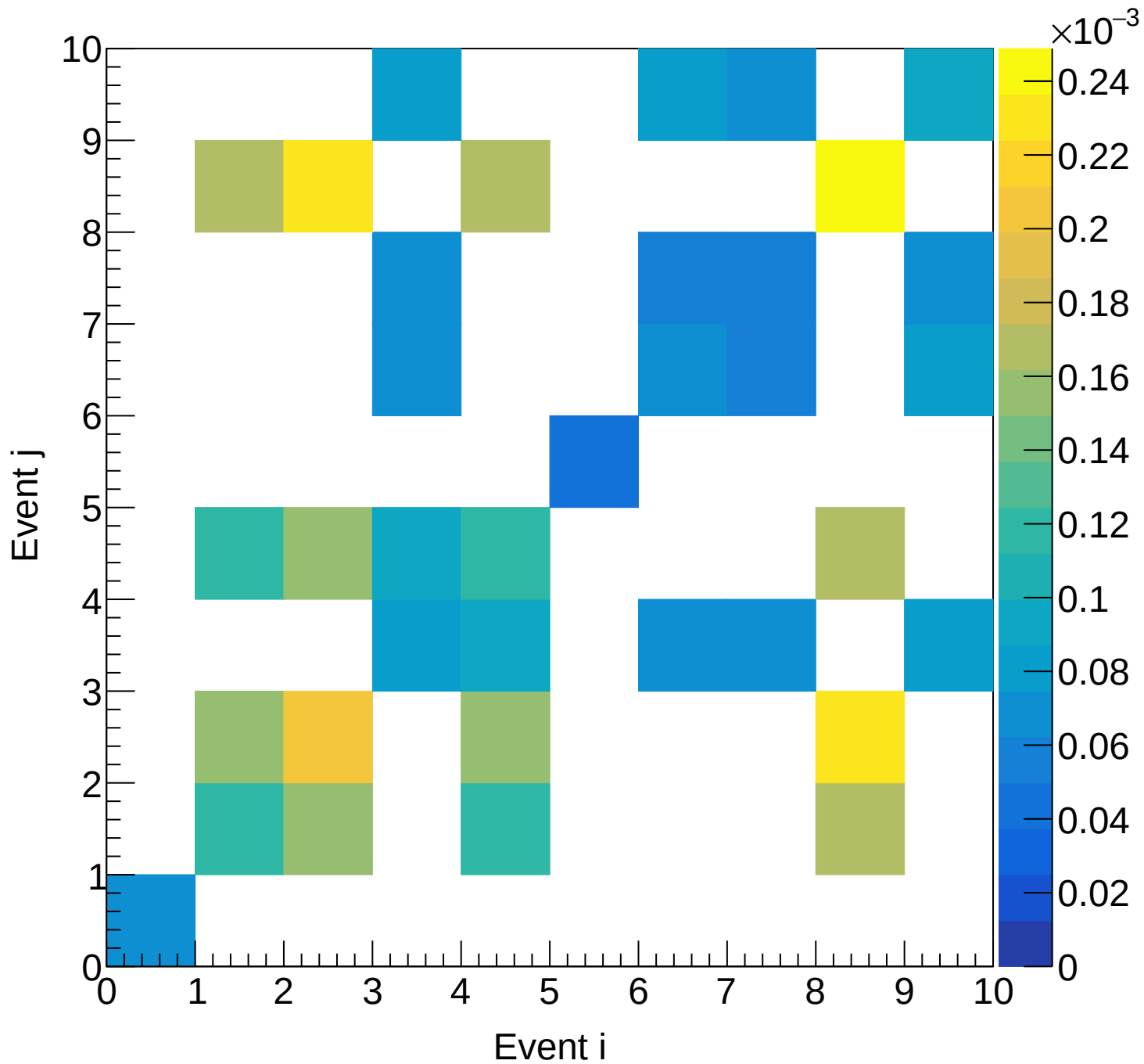
Flask (total) Covariance | M: [5.1, 5.4) xF: [0.15, 0.20)
