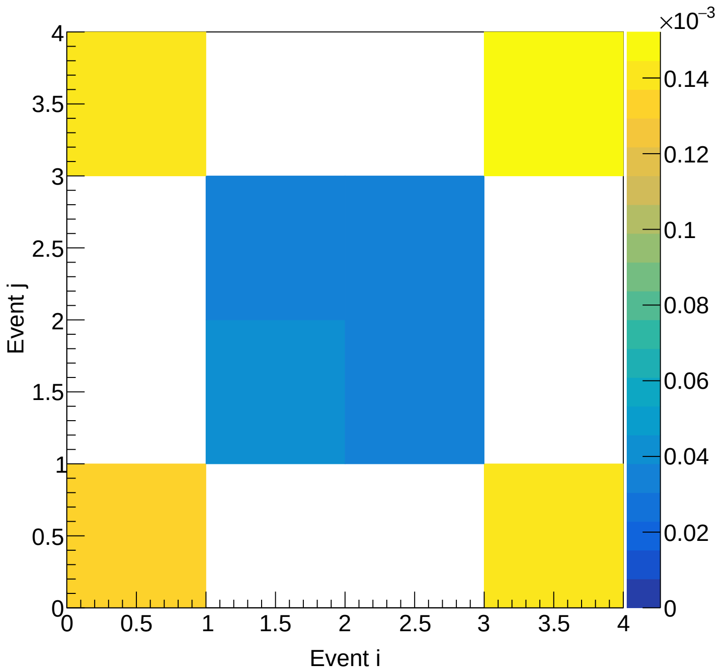
Flask (total) Covariance | M: [5.4, 5.7) xF: [0.15, 0.20)
