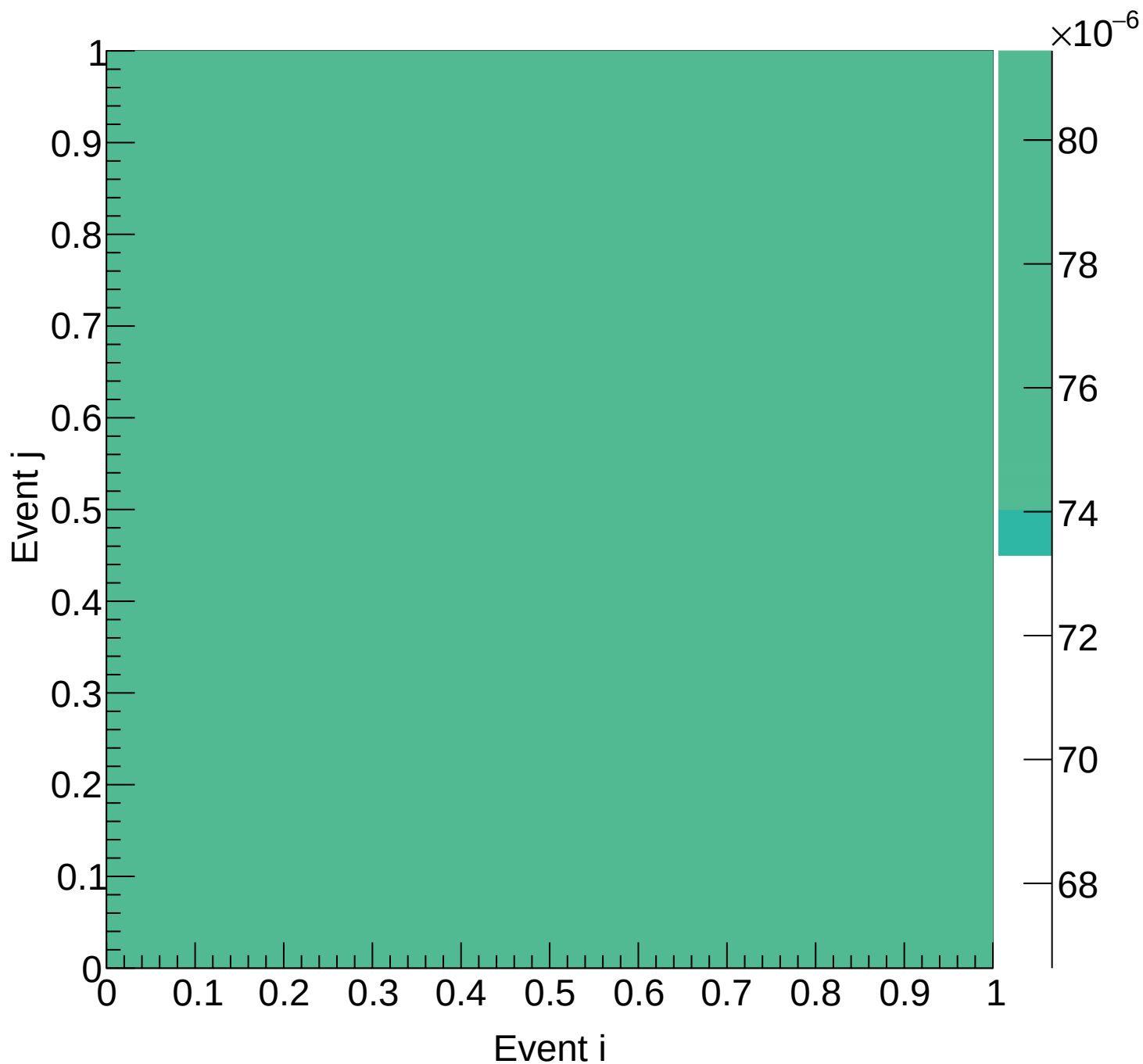
Flask (total) Covariance | M: [6.9, 7.5) xF: [0.20, 0.25)
