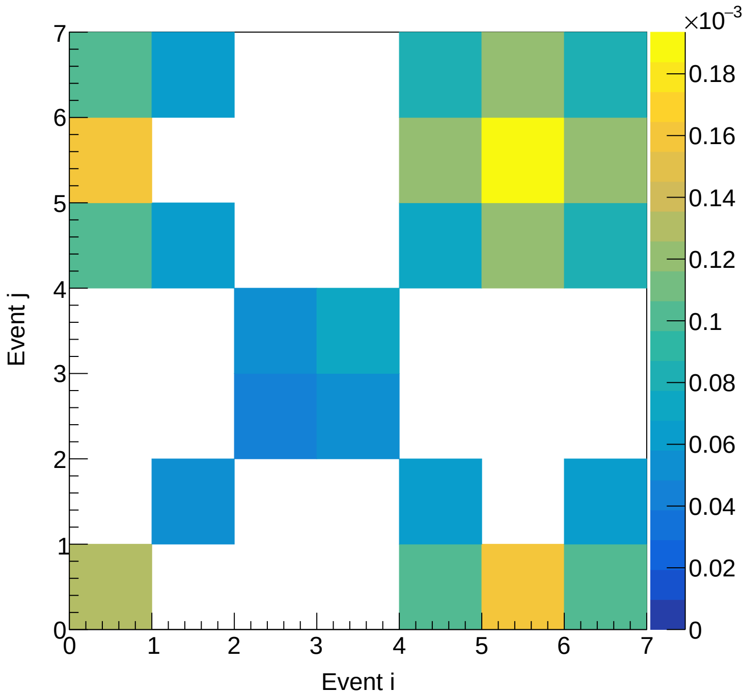
Flask (total) Covariance | M: [4.8, 5.1) xF: [0.20, 0.25)
