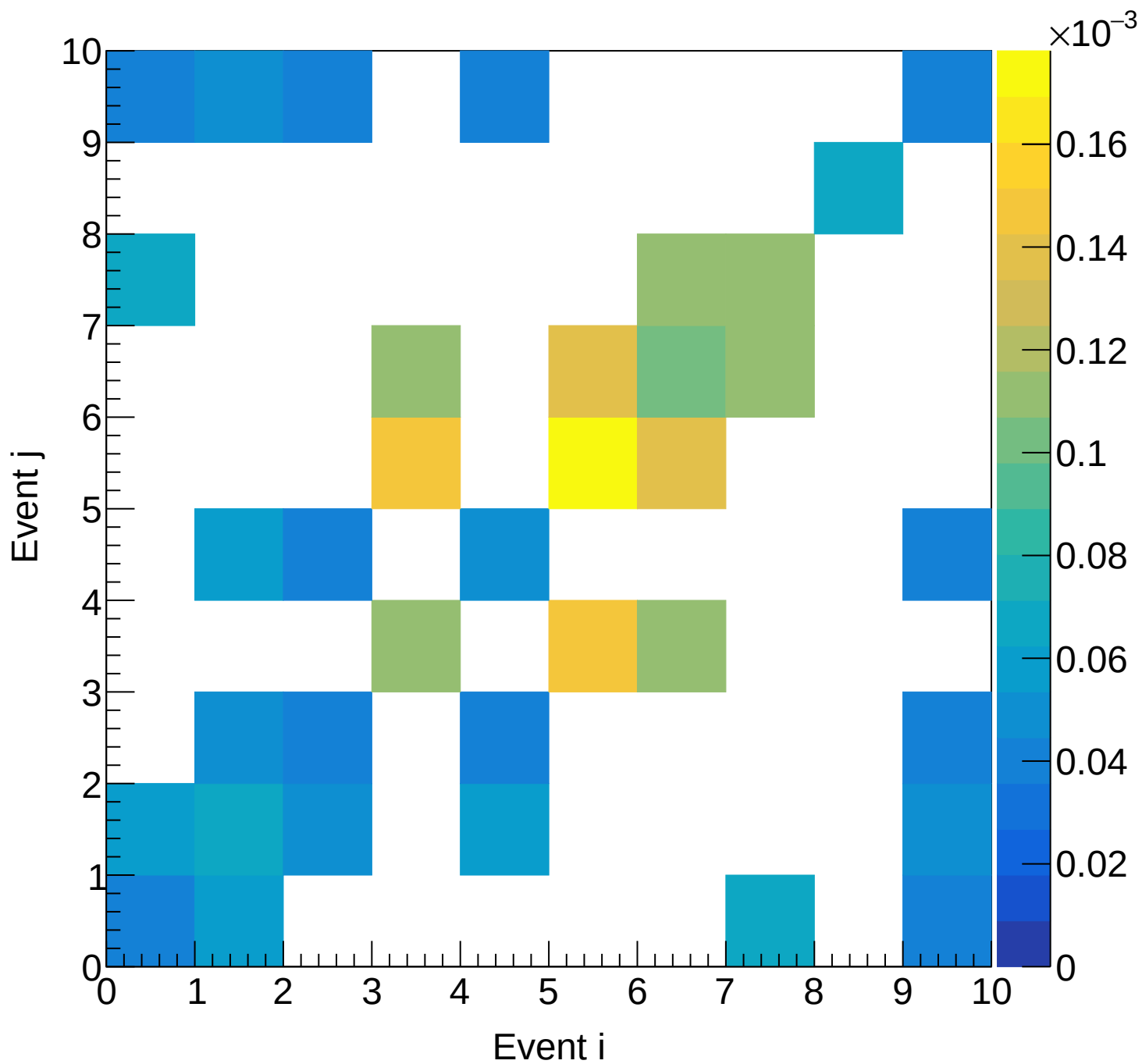
Flask (total) Covariance | M: [5.1, 5.4) xF: [0.20, 0.25)
