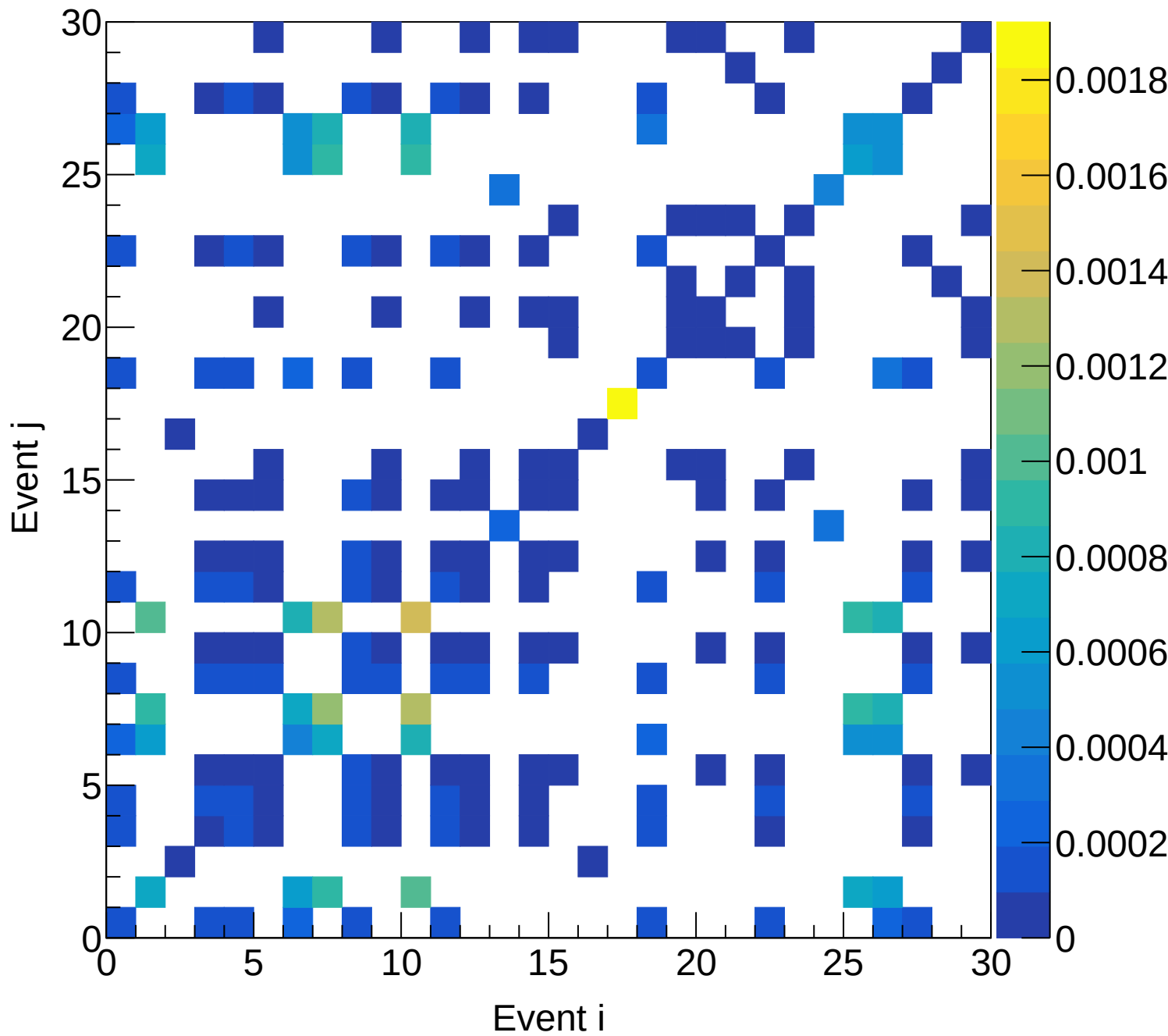
Flask (total) Covariance | M: [4.2, 4.5) xF: [0.30, 0.35)
