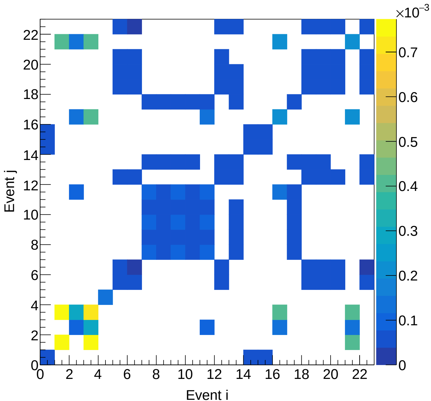
Flask (total) Covariance | M: [4.5, 4.8) xF: [0.30, 0.35)
