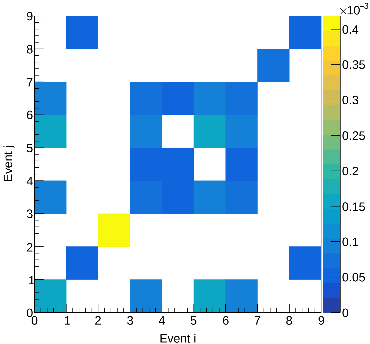
Flask (total) Covariance | M: [4.8, 5.1) xF: [0.30, 0.35)
