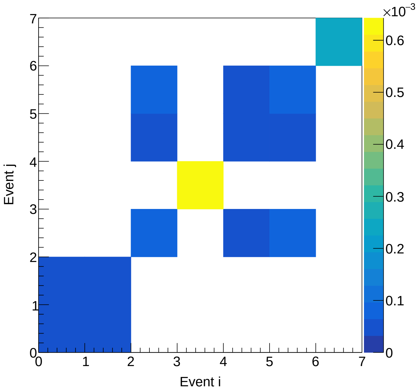
Flask (total) Covariance | M: [5.4, 5.7) xF: [0.30, 0.35)
