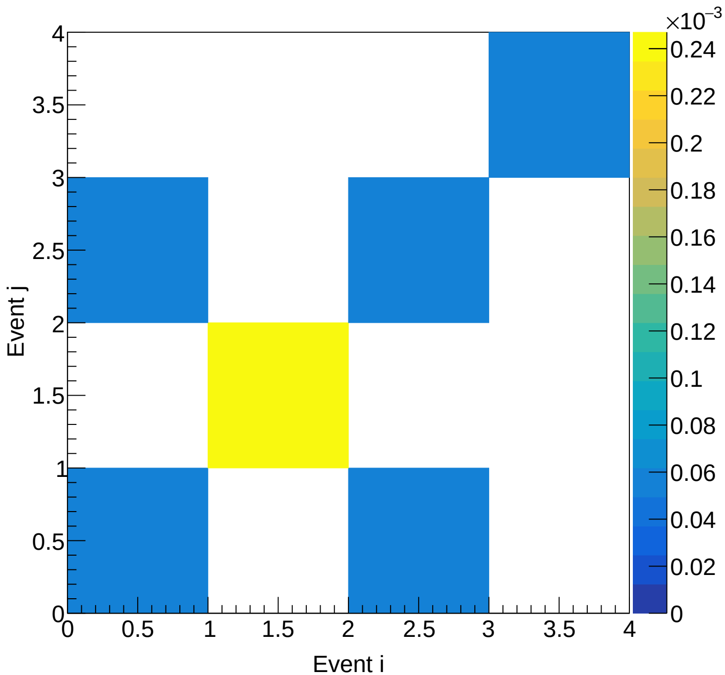
Flask (total) Covariance | M: [6.3, 6.6) xF: [0.35, 0.40)
