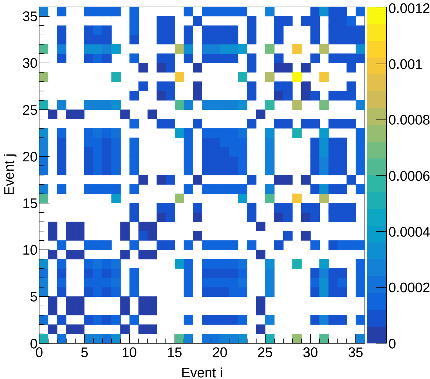
Flask (total) Covariance | M: [3.9, 4.2) xF: [0.35, 0.40)
