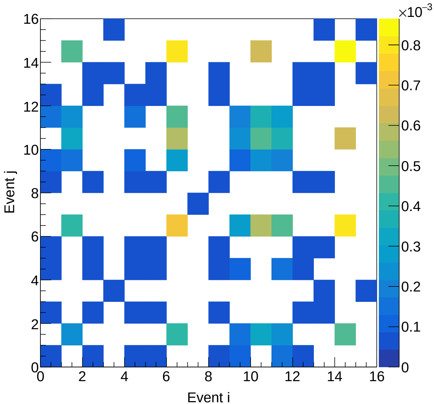
Flask (total) Covariance | M: [4.5, 4.8) xF: [0.35, 0.40)
