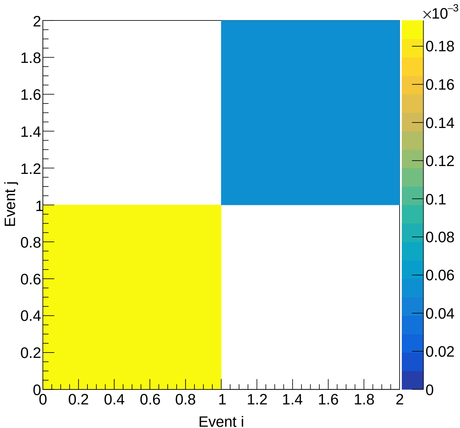
Flask (total) Covariance | M: [5.7, 6.0) xF: [0.35, 0.40)
