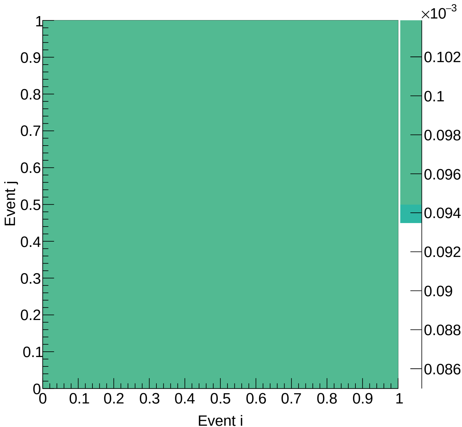
Flask (total) Covariance | M: [6.9, 7.5) xF: [0.40, 0.45)
