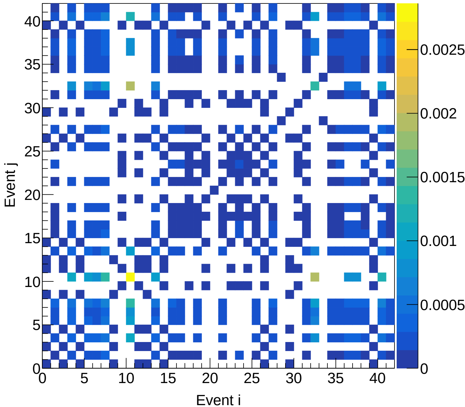
Flask (total) Covariance | M: [3.9, 4.2) xF: [0.40, 0.45)
