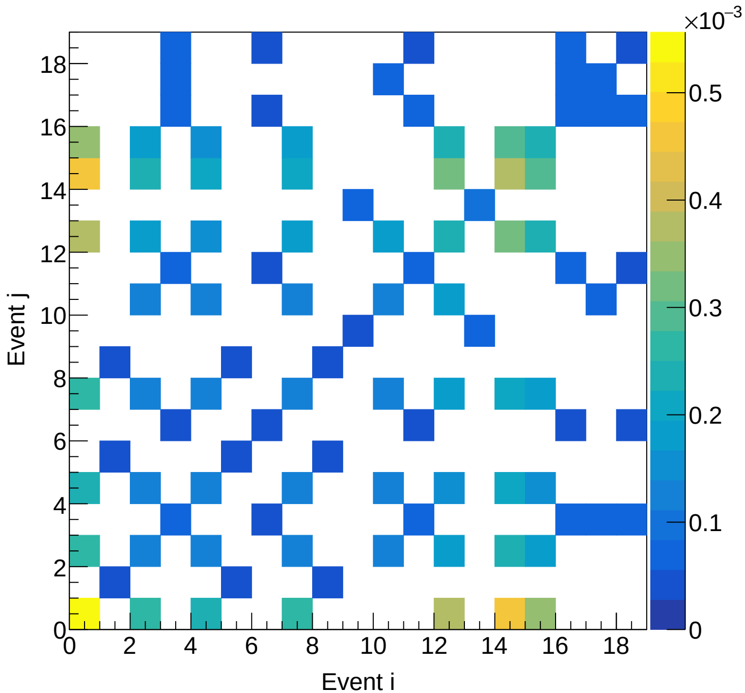
Flask (total) Covariance | M: [4.5, 4.8) xF: [0.40, 0.45)
