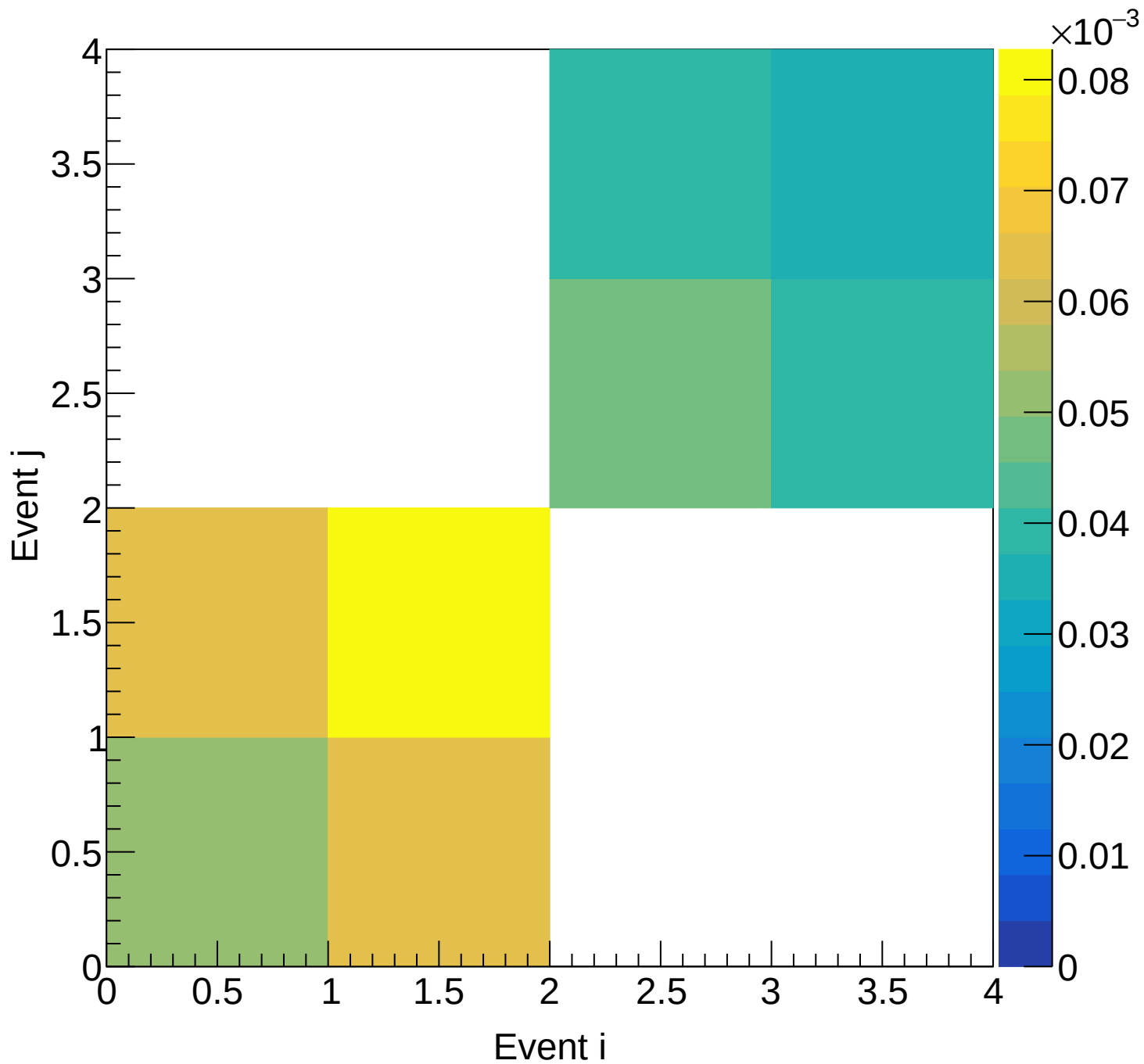
LD2 (mix) Covariance | M: [5.1, 5.4] xF: [-0.05, 0.00]
