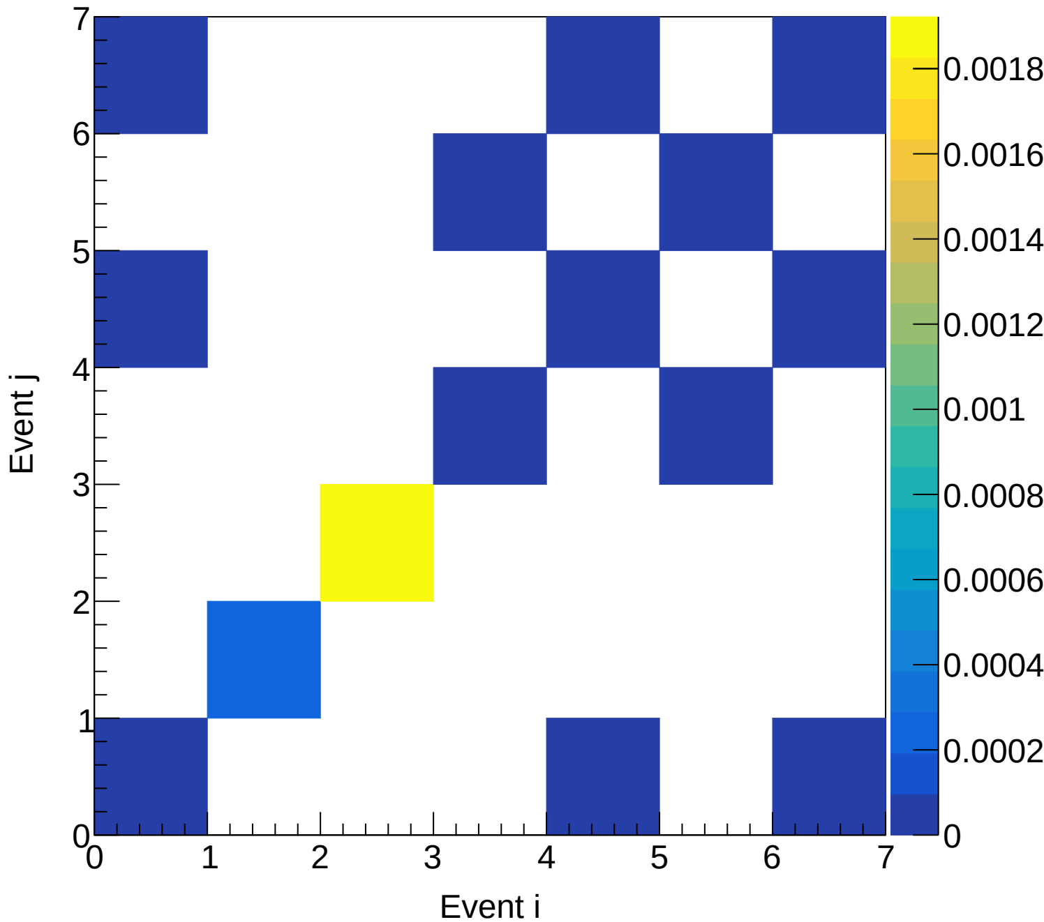
LD2 (mix) Covariance | M: [5.4, 5.7) xF: [-0.05, 0.00)
