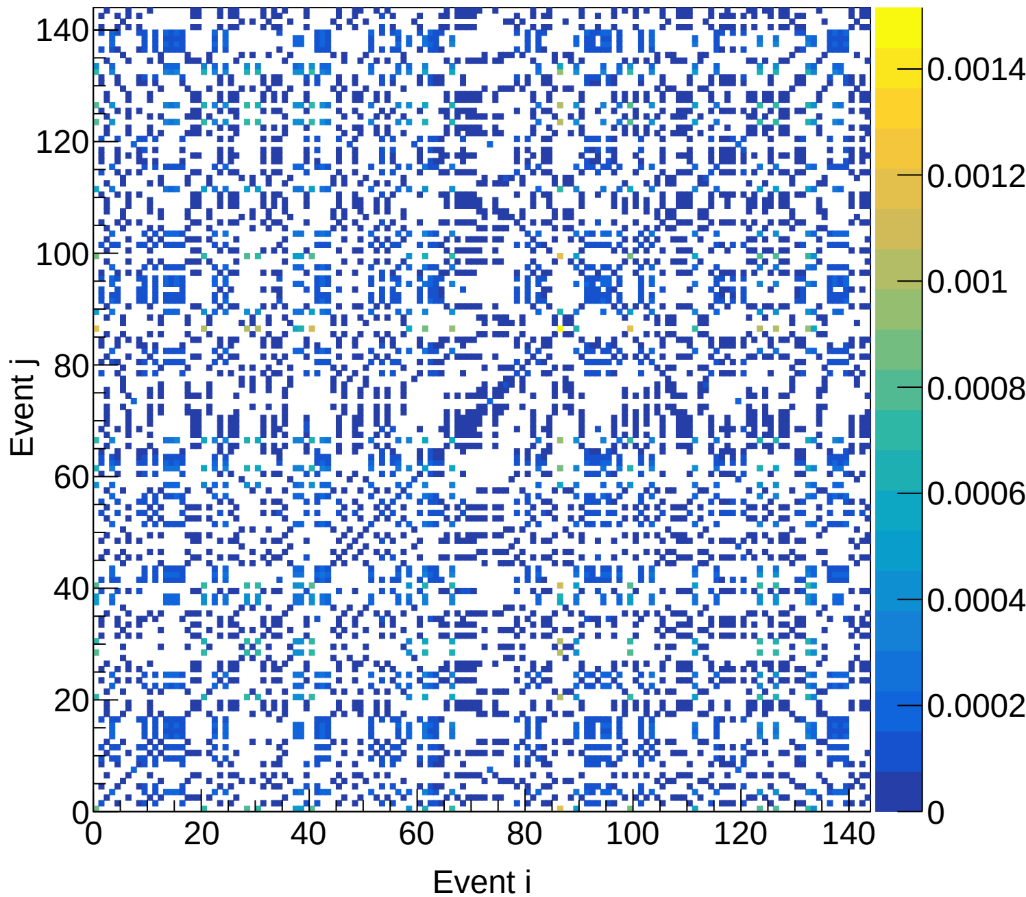
LD2 (mix) Covariance | M: [3.9, 4.2) xF: [0.45, 0.50)
