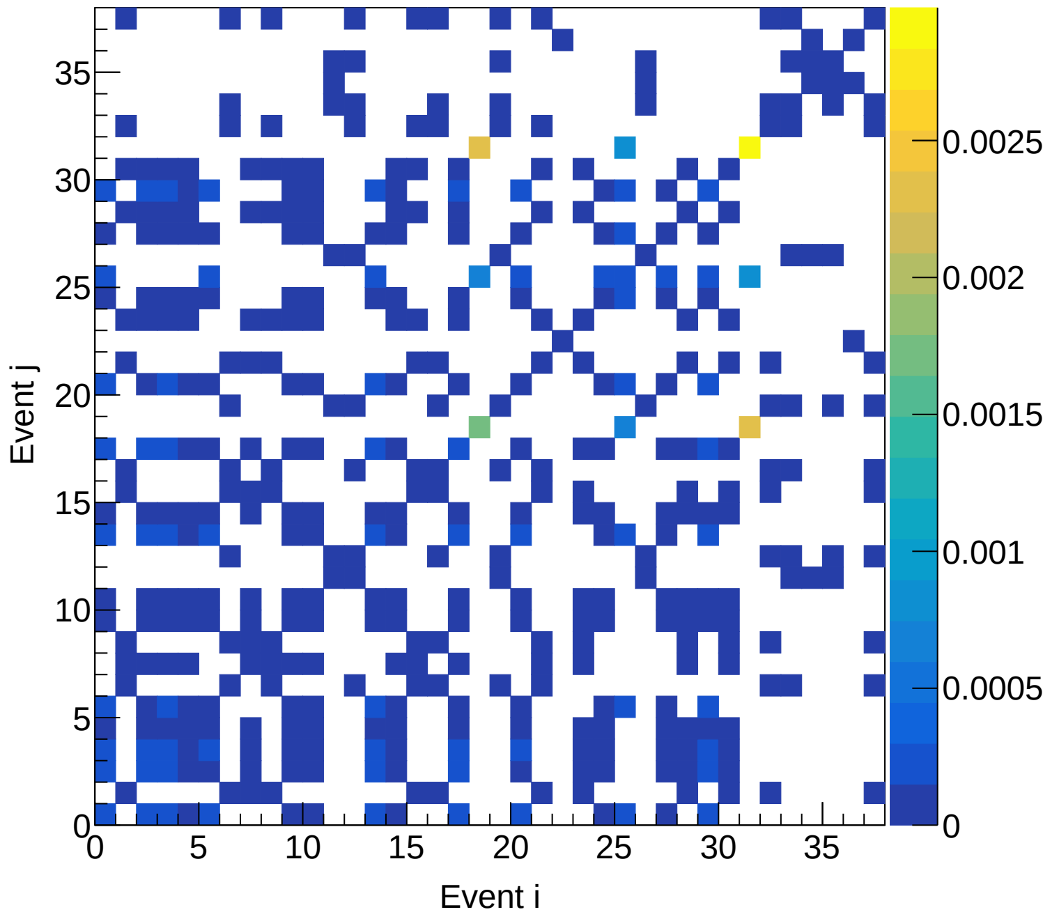
LD2 (mix) Covariance | M: [4.5, 4.8) xF: [0.45, 0.50)
