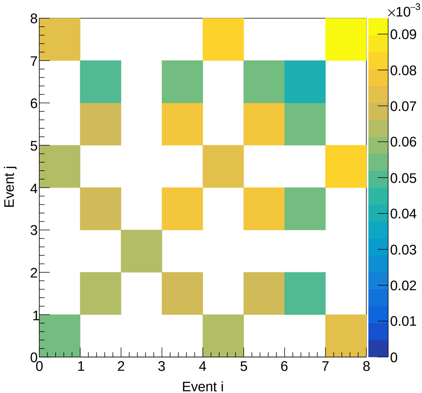
LD2 (mix) Covariance | M: [5.4, 5.7) xF: [0.45, 0.50)
