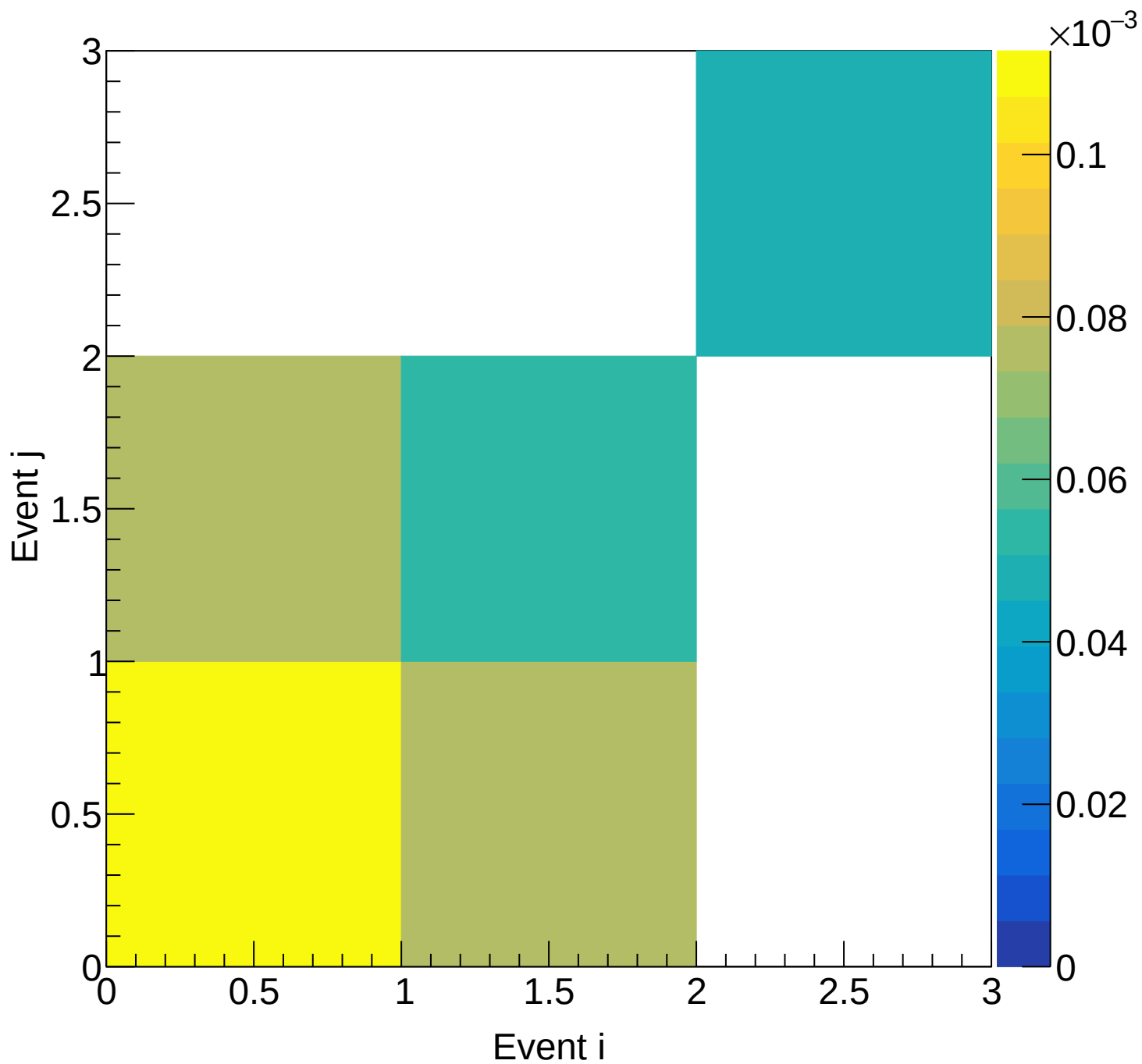
LD2 (mix) Covariance | M: [5.7, 6.0] xF: [0.45, 0.50)
