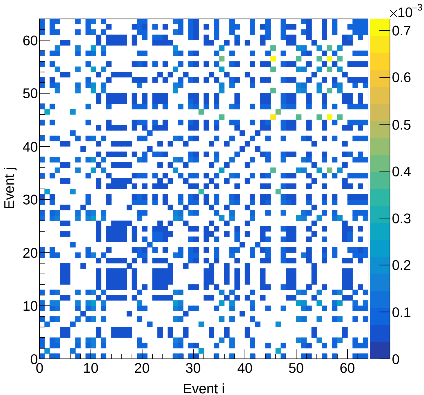
LD2 (mix) Covariance | M: [4.2, 4.5) xF: [0.50, 0.55)
