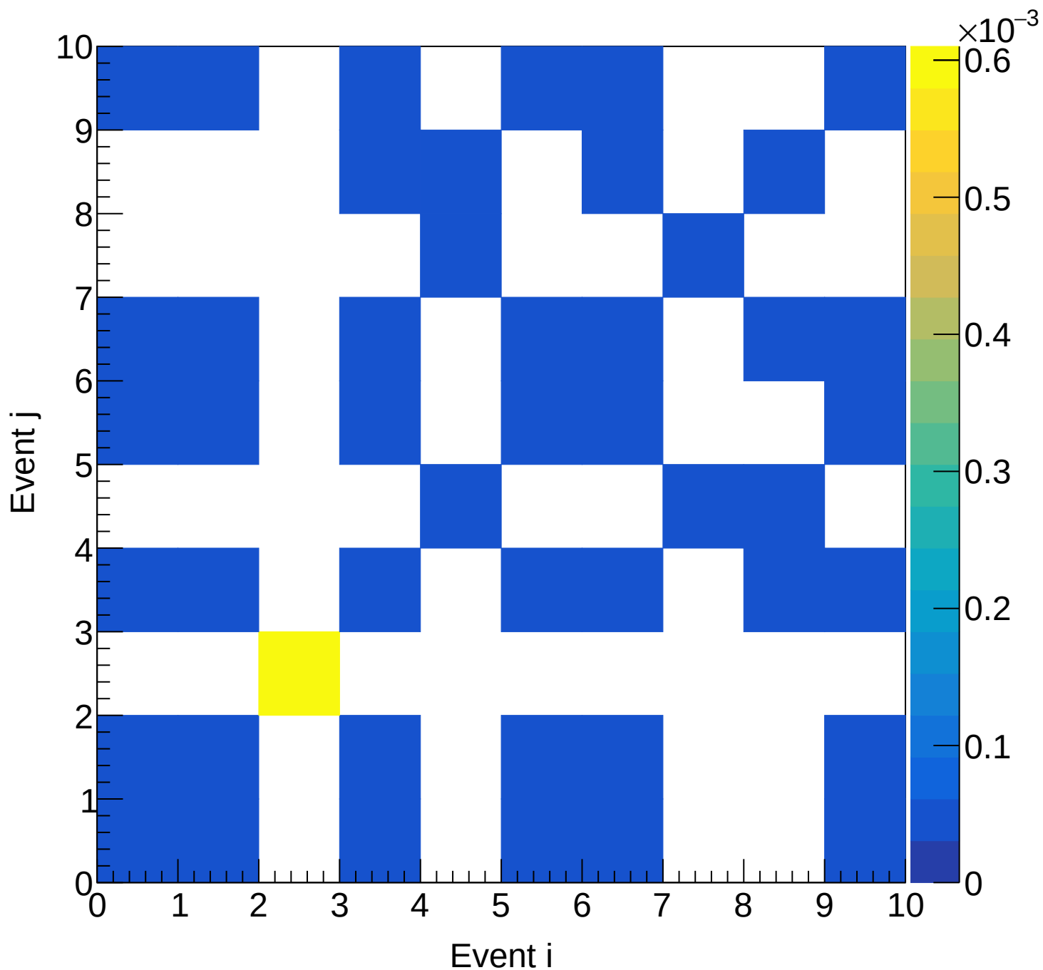
LD2 (mix) Covariance | M: [4.8, 5.1] xF: [0.50, 0.55)
