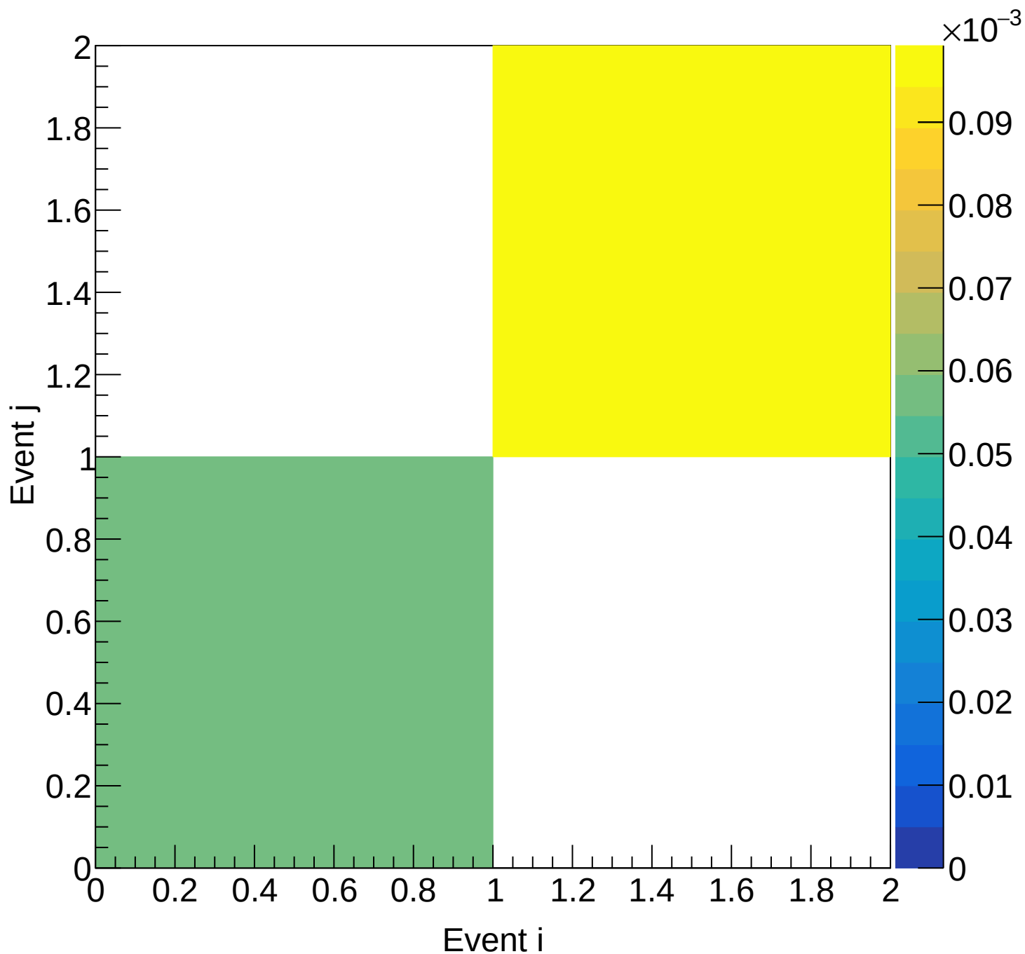
LD2 (mix) Covariance | M: [5.1, 5.4) xF: [0.55, 0.60)
