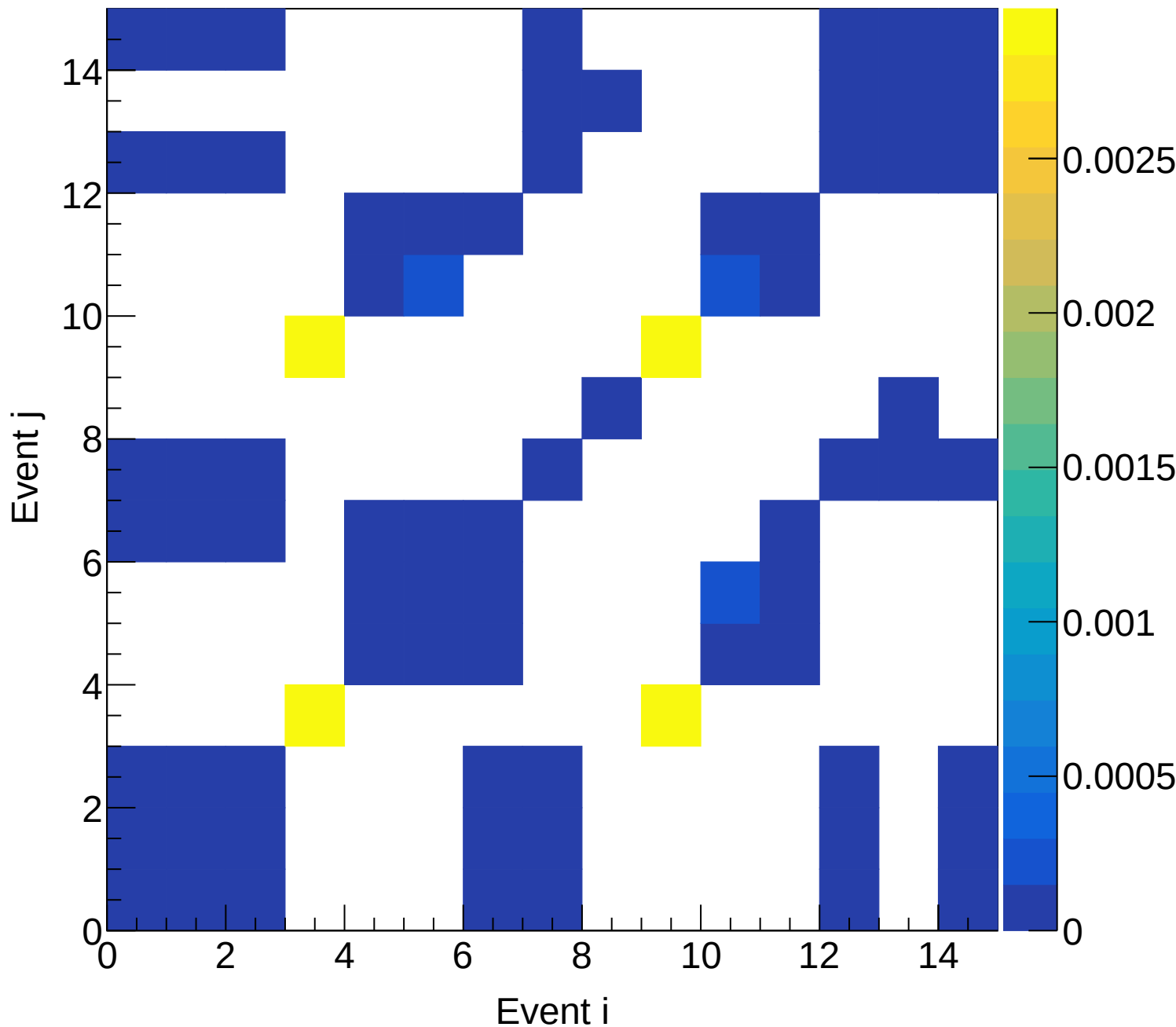
LD2 (mix) Covariance | M: [4.5, 4.8) xF: [0.60, 0.65)
