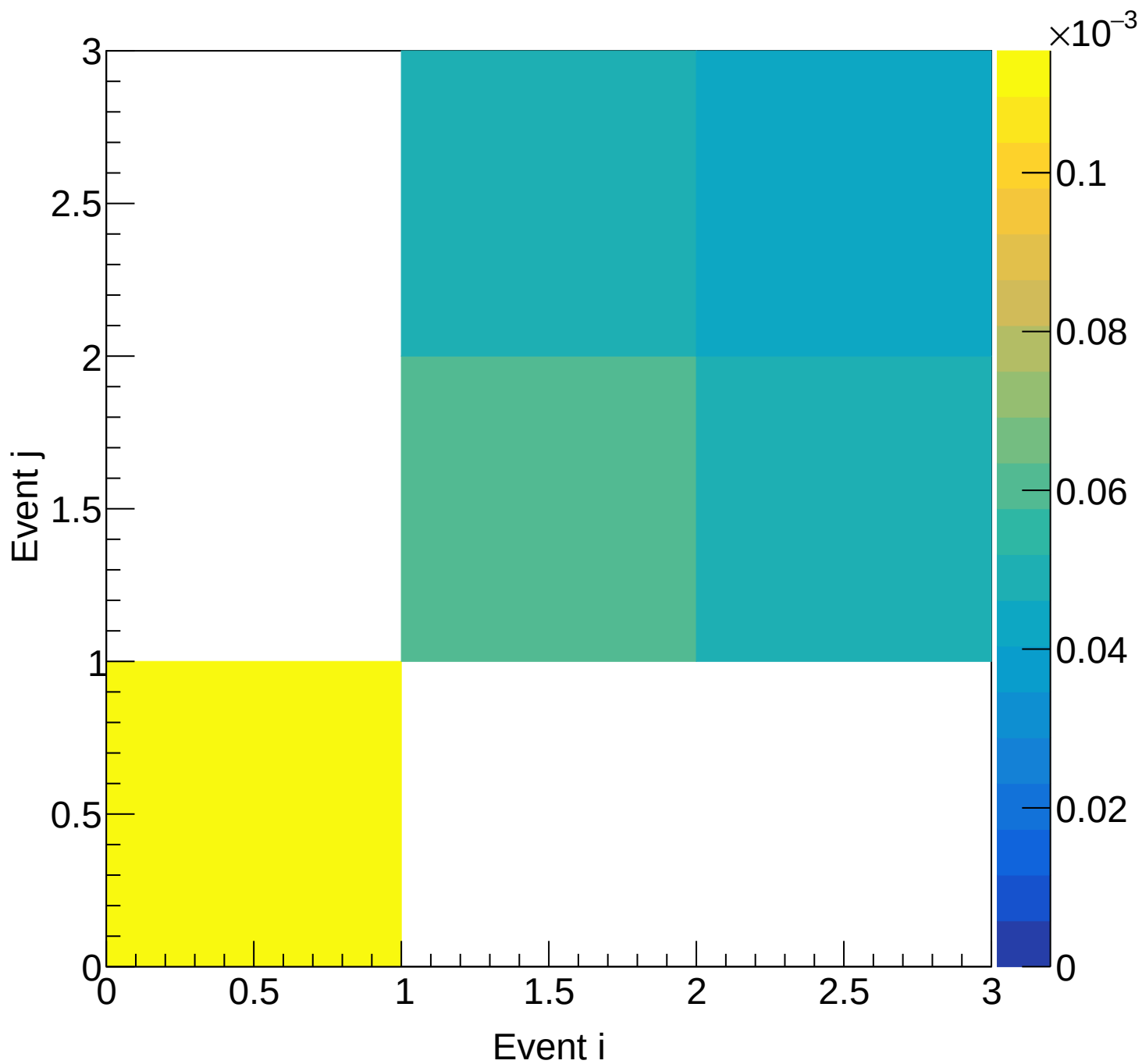
LD2 (mix) Covariance | M: [5.1, 5.4) xF: [0.60, 0.65)
