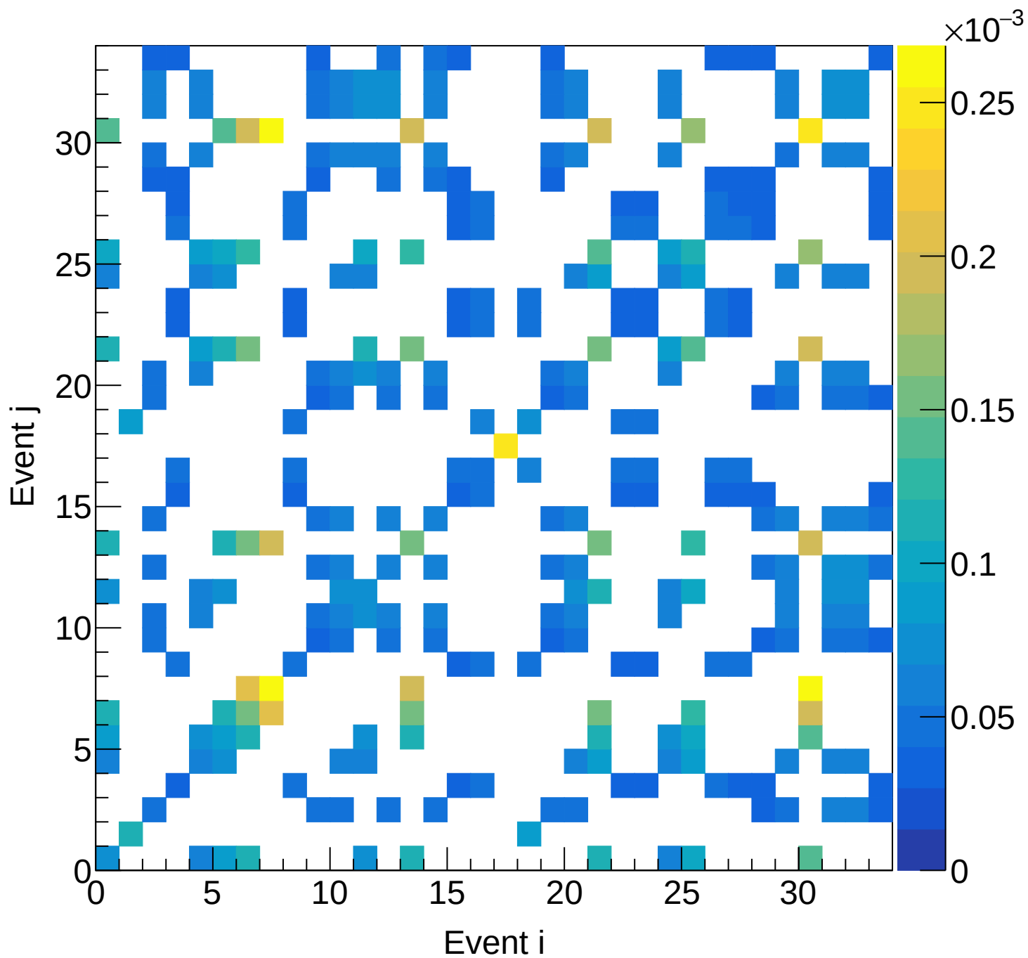
LD2 (mix) Covariance | M: [4.2, 4.5) xF: [0.65, 0.70)
