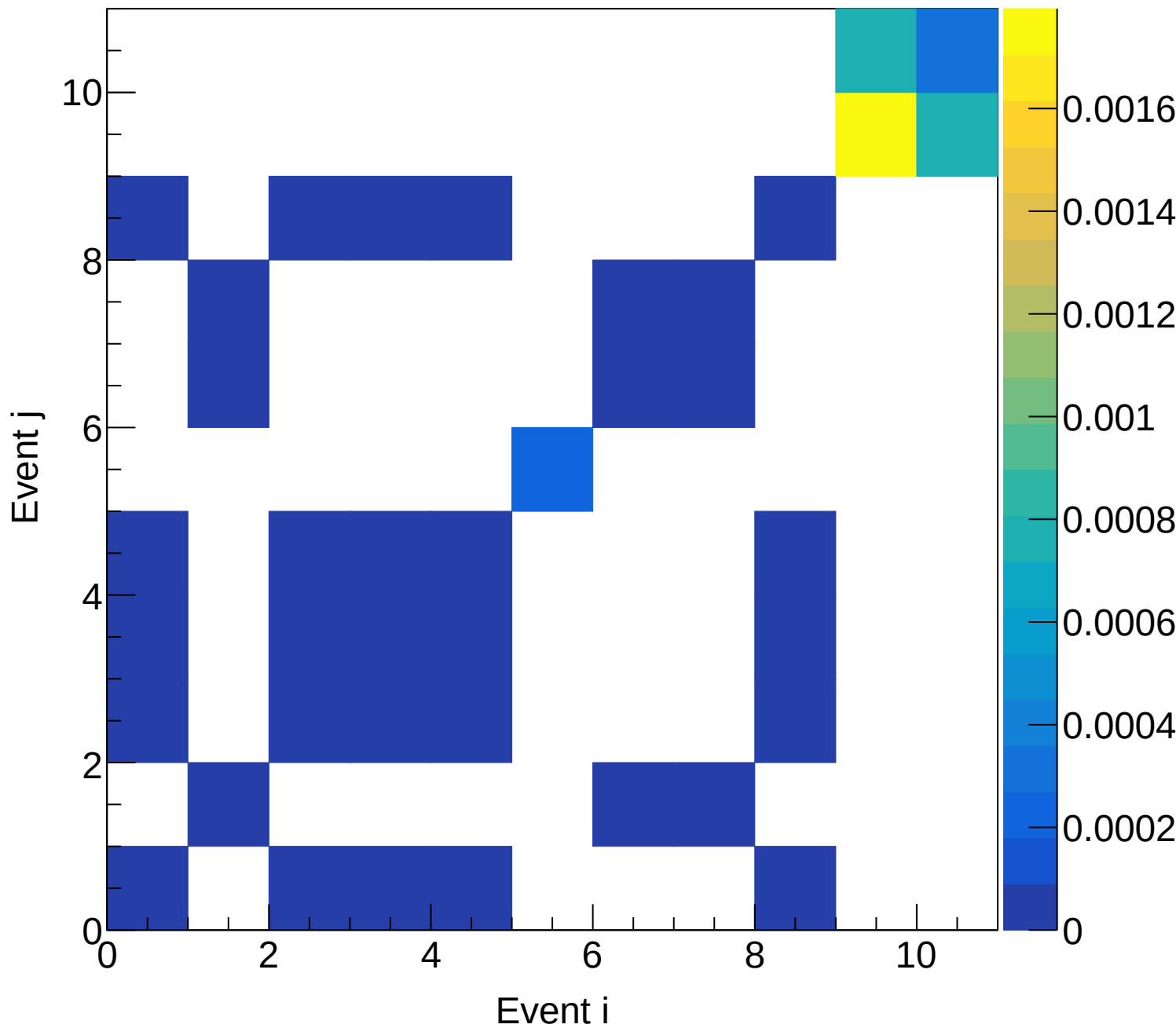
LD2 (mix) Covariance | M: [4.5, 4.8) xF: [0.65, 0.70)
