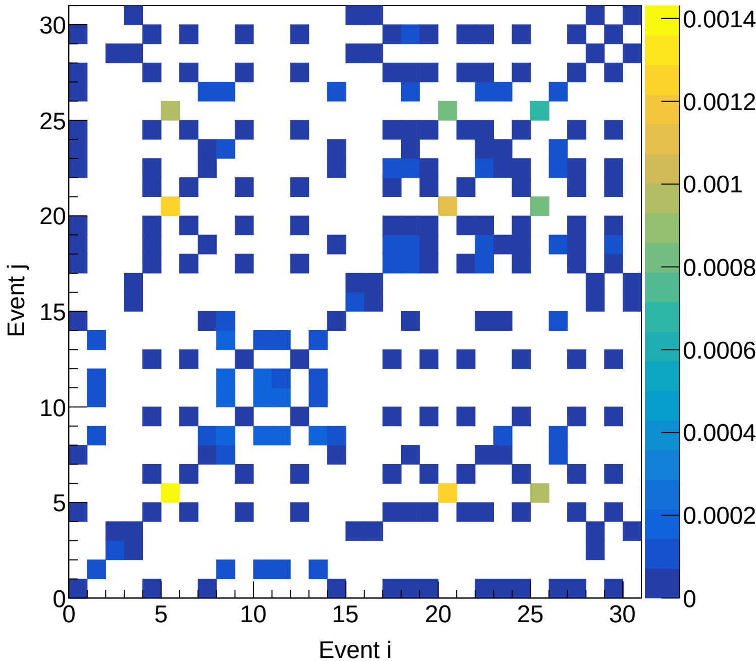
LD2 (mix) Covariance | M: [3.9, 4.2] xF: [0.70, 0.75)
