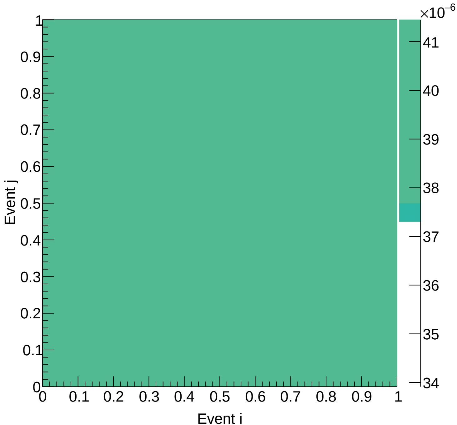
LD2 (mix) Covariance | M: [5.4, 5.7) xF: [0.70, 0.75)
