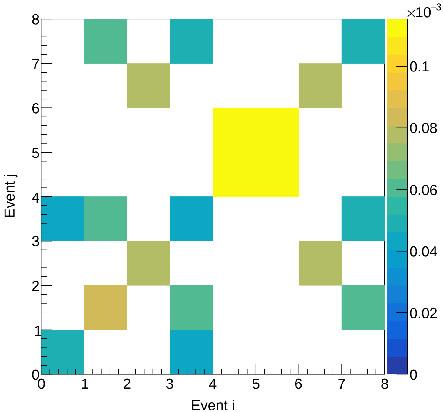
LD2 (mix) Covariance | M: [5.1, 5.4) xF: [0.00, 0.05)
