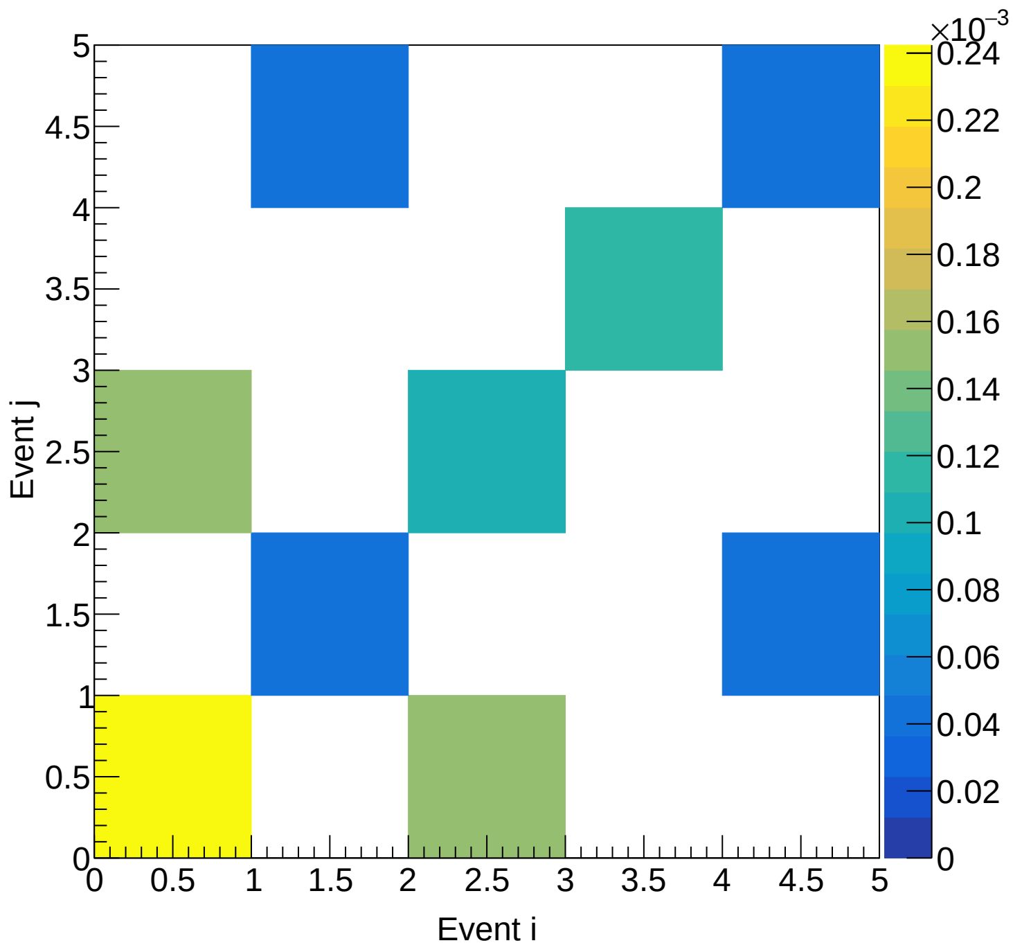
LD2 (mix) Covariance | M: [5.4, 5.7) xF: [0.00, 0.05)
