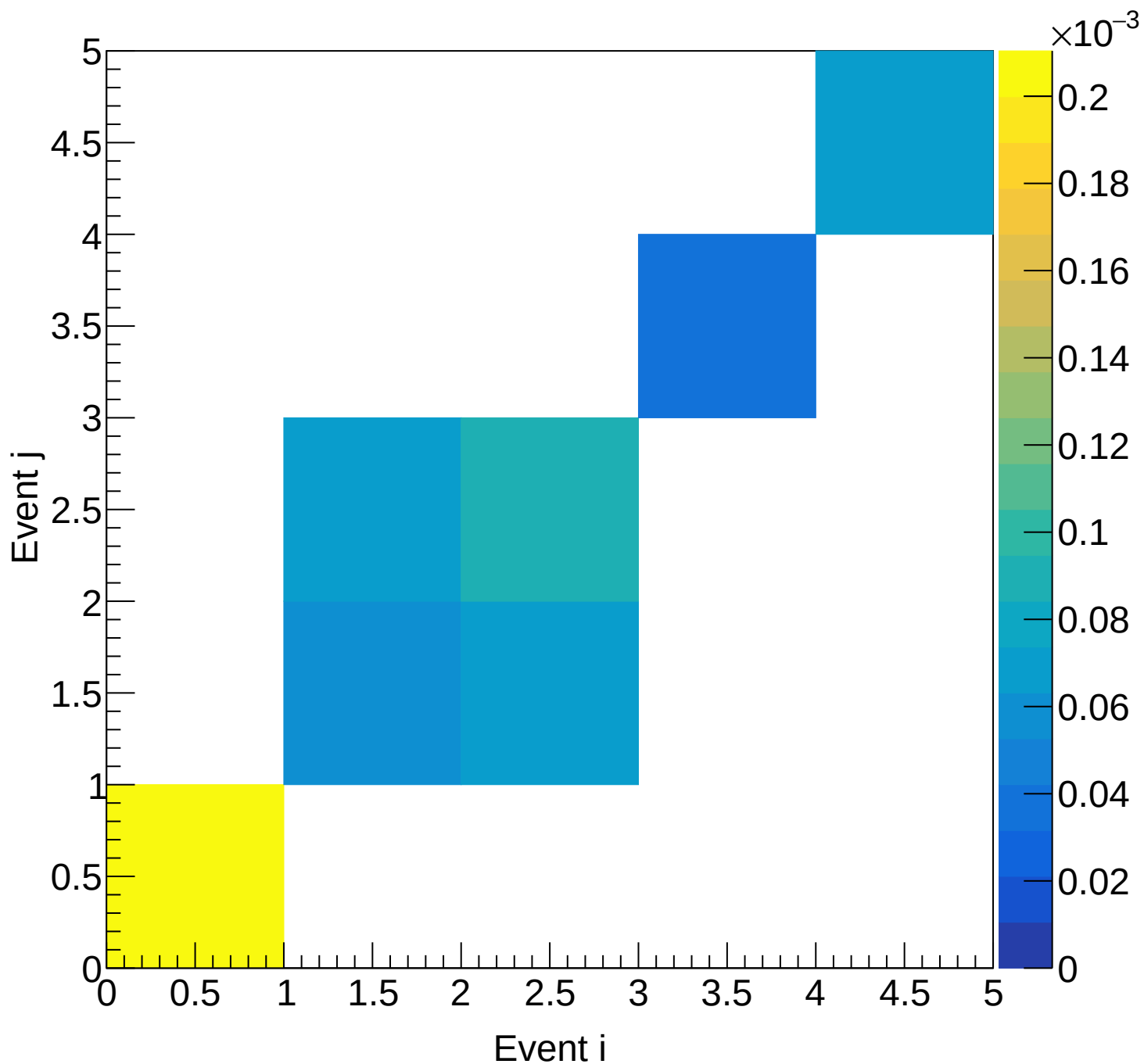
LD2 (mix) Covariance | M: [4.5, 4.8) xF: [0.05, 0.10)
